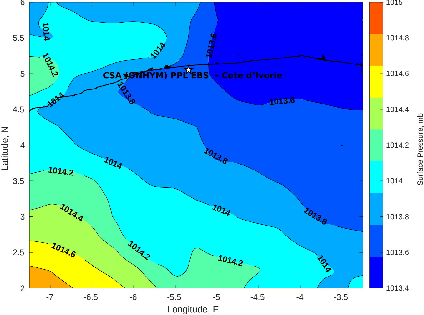
Surface Pressure (mb) for CSA (ONHYM) PPL EBS - Cote d'Ivoire at 02-Nov-2025 00:00:00
