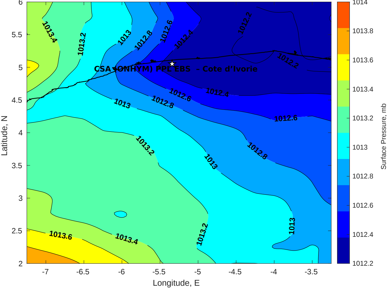
Surface Pressure (mb) for CSA (ONHYM) PPL EBS - Cote d'Ivoire at 03-Nov-2025 00:00:00
