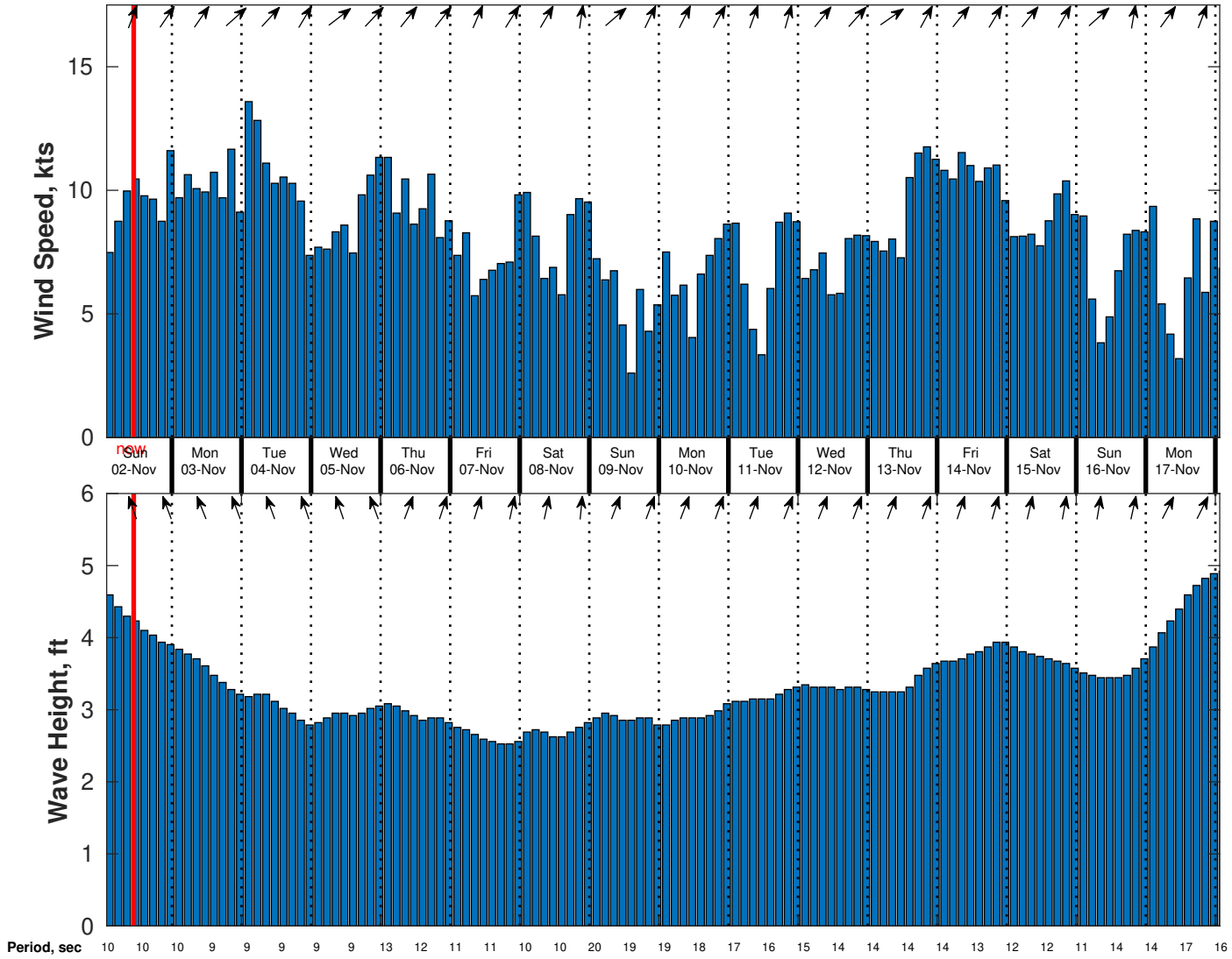
Wind & Wave Forecast for CSA (ONHYM) PPL EBS - Cote d'Ivoire from 01-Nov-2025 01:00:00 to 17-Nov-2025 01:00:00
