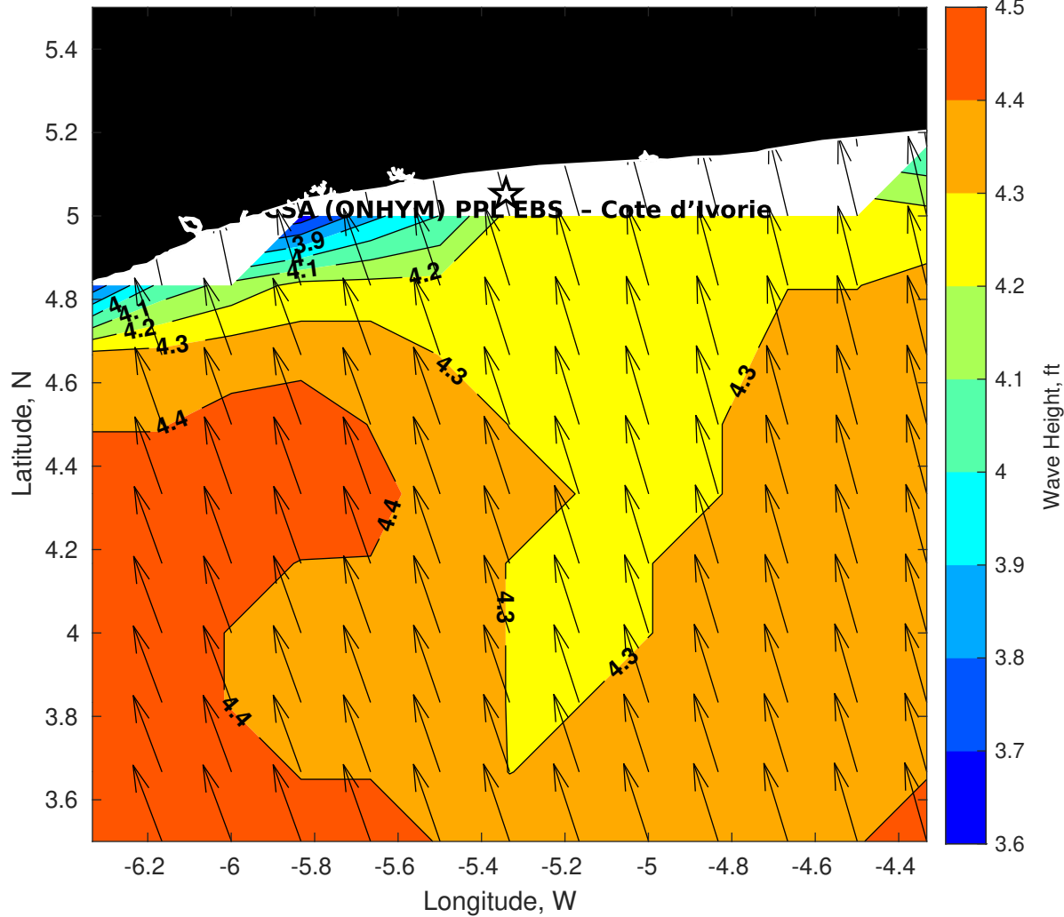
Wave Height (ft) for CSA (ONHYM) PPL EBS - Cote d'Ivoire at 01-Nov-2025 09:00:00
