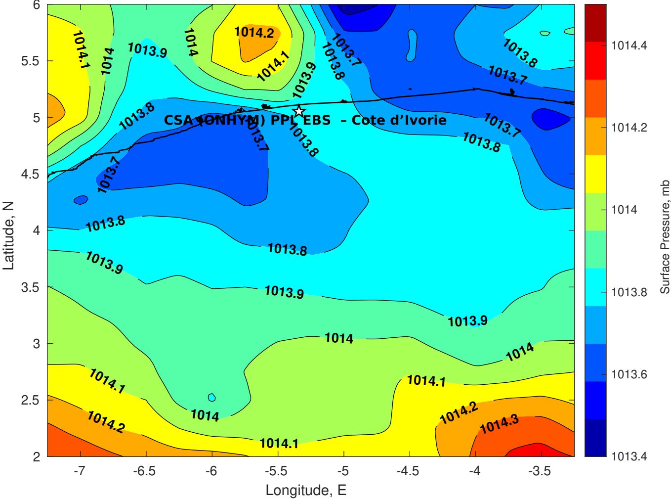
Surface Pressure (mb) for CSA (ONHYM) PPL EBS - Cote d'Ivoire at 01-Nov-2025 00:00:00
