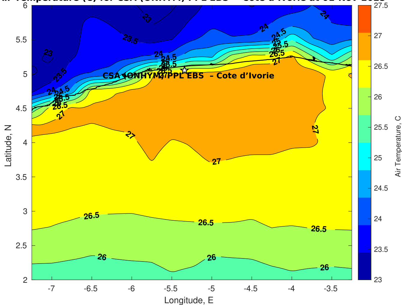
Air Temperature (C) for CSA (ONHYM) PPL EBS - Cote d'Ivoire at 01-Nov-2025
