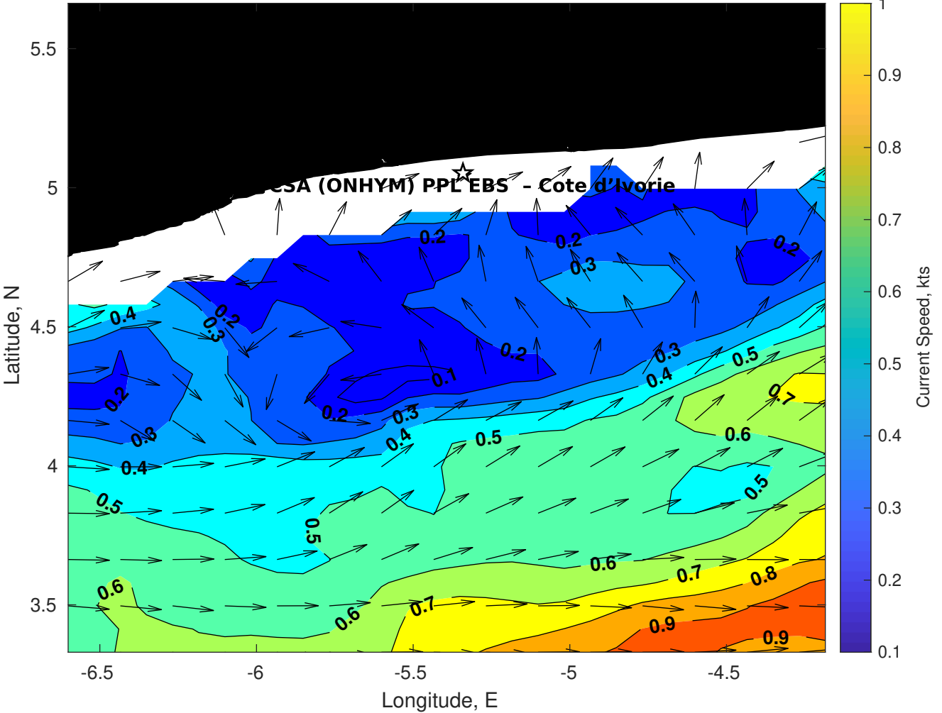
Surface Currents for CSA (ONHYM) PPL EBS - Cote d'Ivoire at 31-Oct-2025 00:00:00
