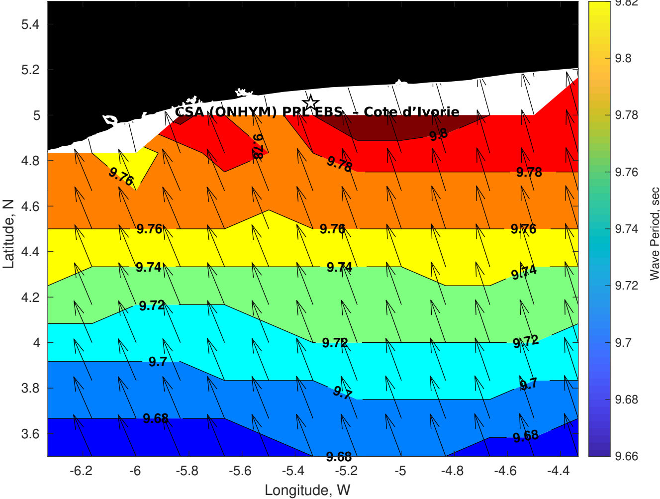
Wave Period (sec) for CSA (ONHYM) PPL EBS - Cote d'Ivoire at 01-Nov-2025 09:00:00
