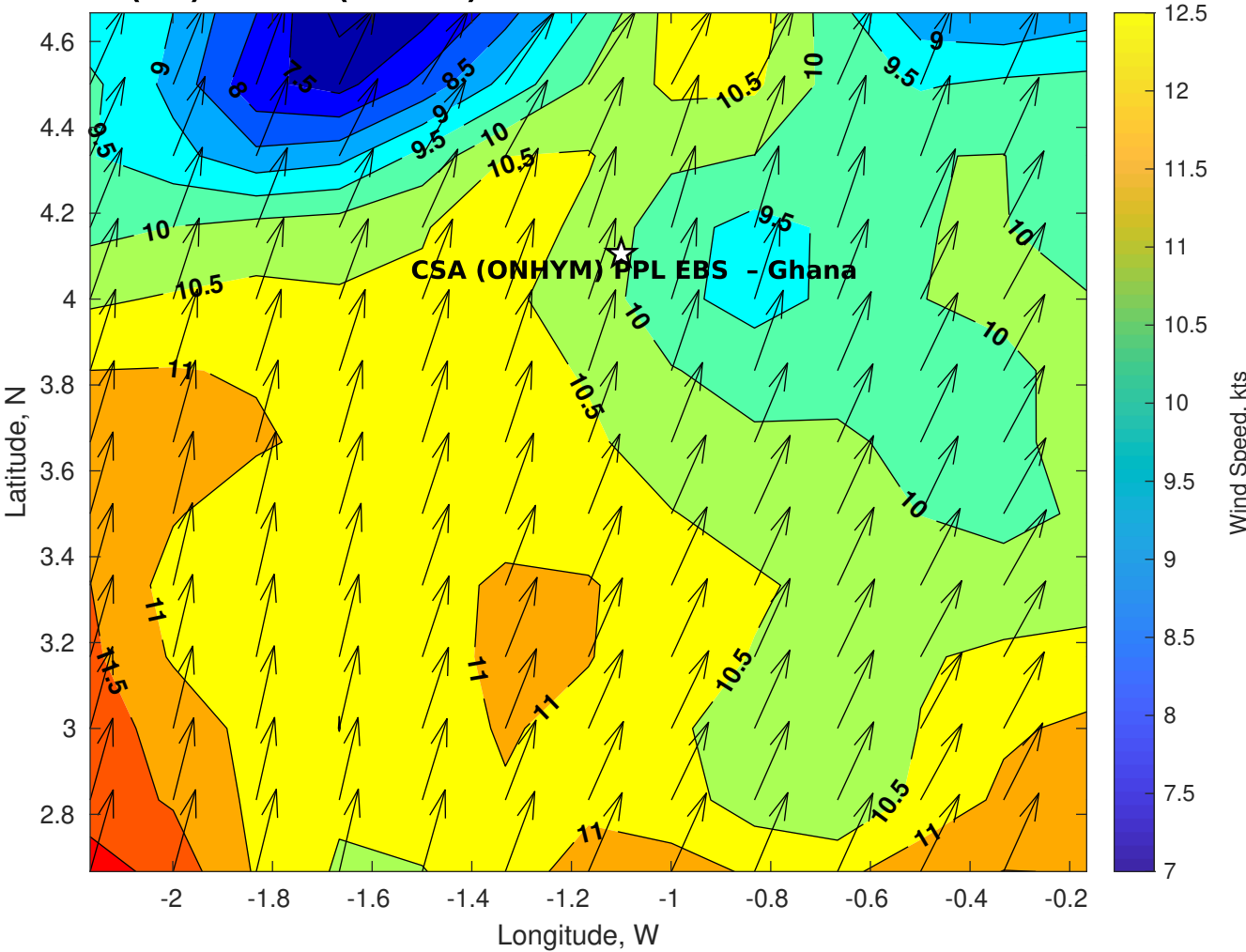
Winds (kts) for CSA (ONHYM) PPL EBS - Ghana at 01-Nov-2025 09:00:00
