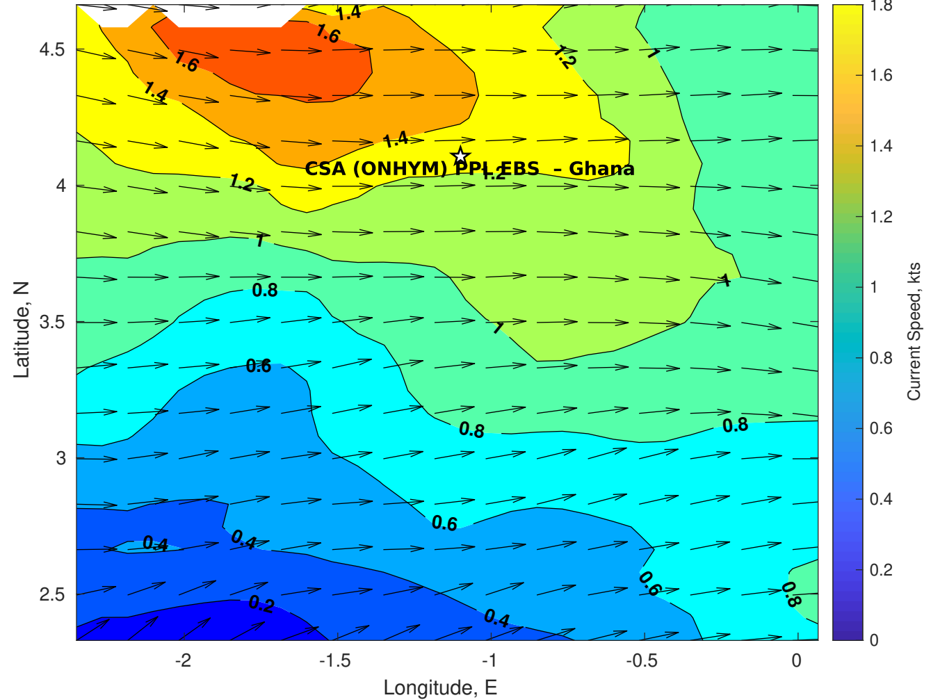
Surface Currents for CSA (ONHYM) PPL EBS - Ghana at 31-Oct-2025 00:00:00
