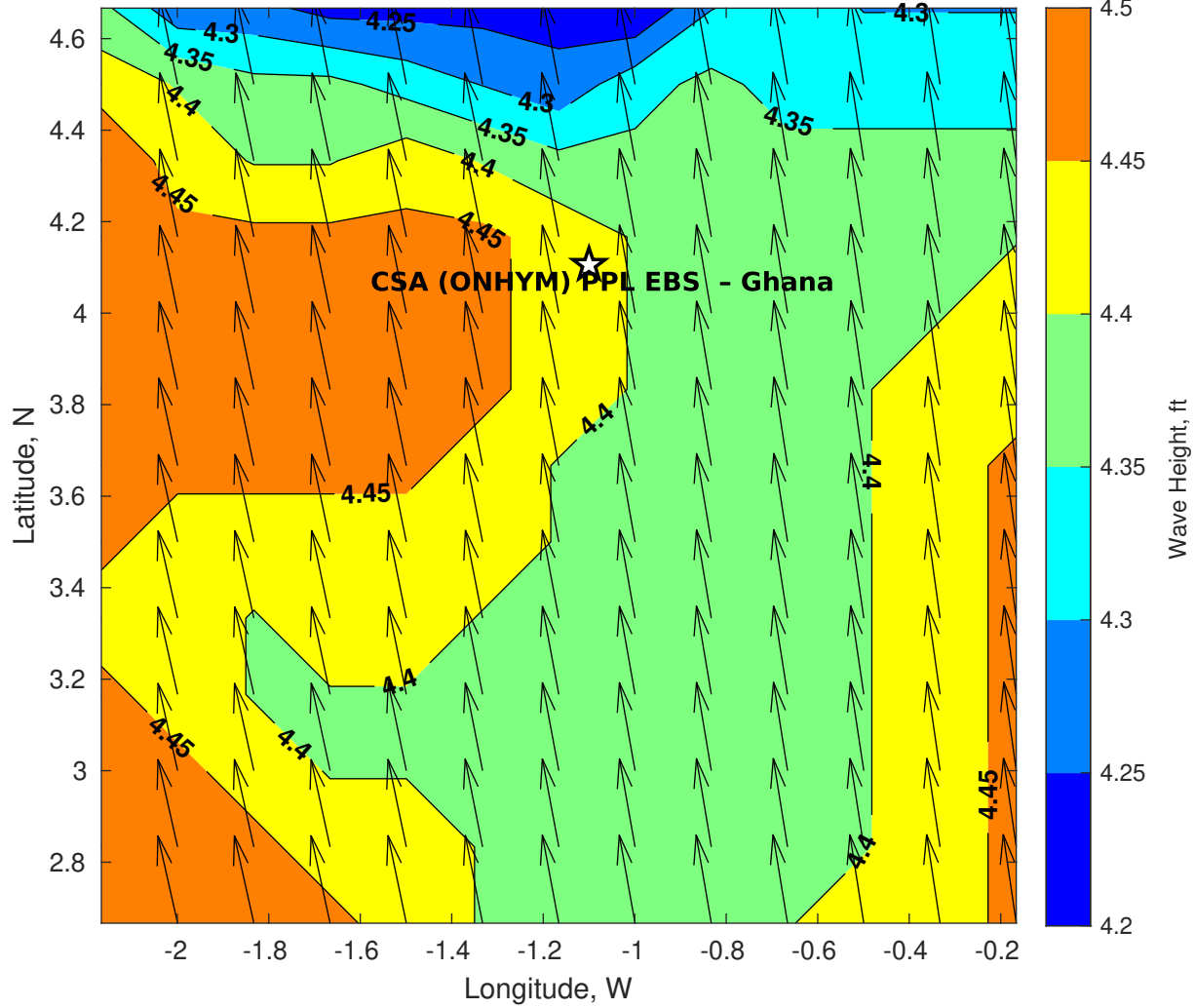
Wave Height (ft) for CSA (ONHYM) PPL EBS - Ghana at 01-Nov-2025 09:00:00
