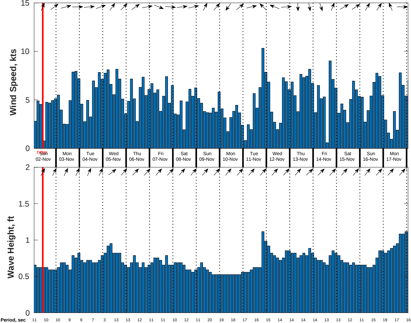
Wind & Wave Forecast for CSA (ONHYM) PPL EBS - Guinea from 01-Nov-2025 01:00:00 to 17-Nov-2025 01:00:00
