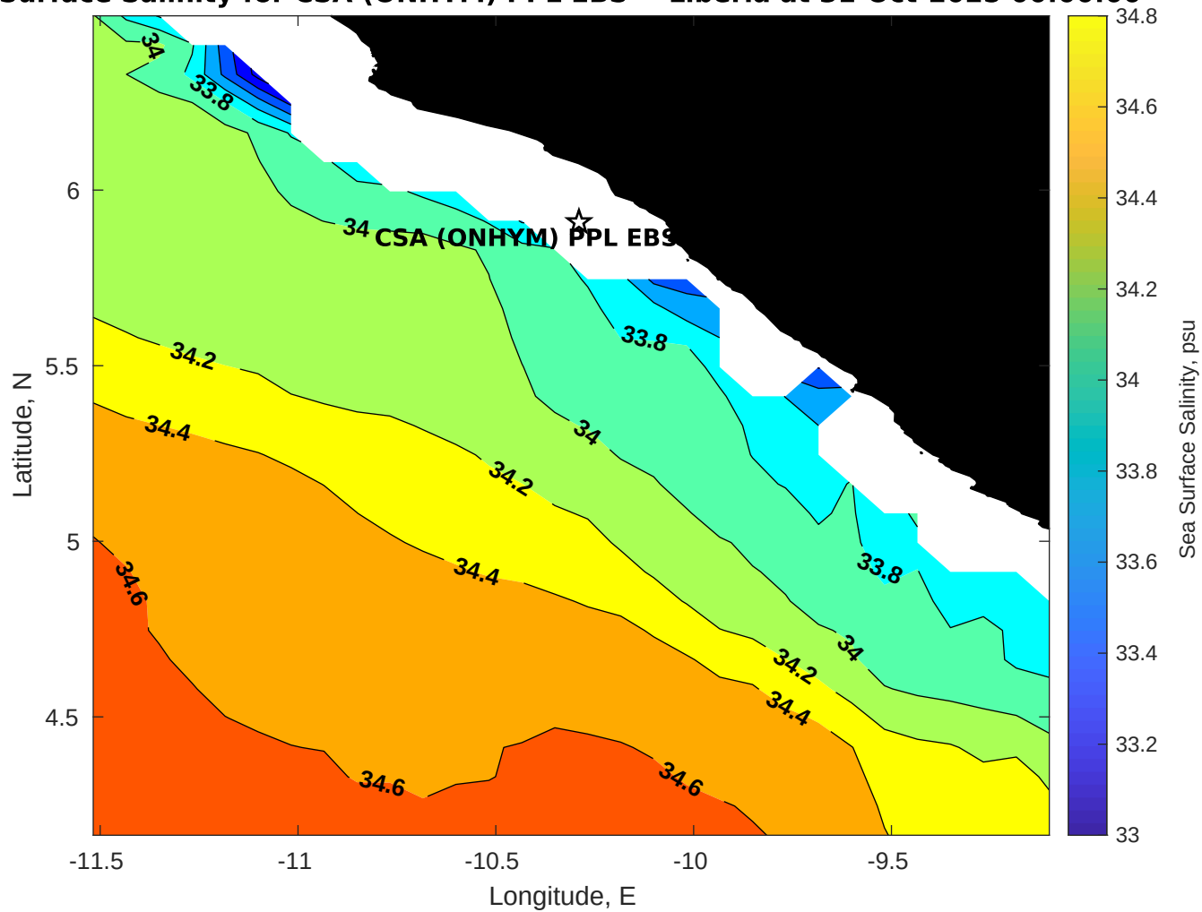
Surface Salinity for CSA (ONHYM) PPL EBS - Liberia at 31-Oct-2025 00:00:00
