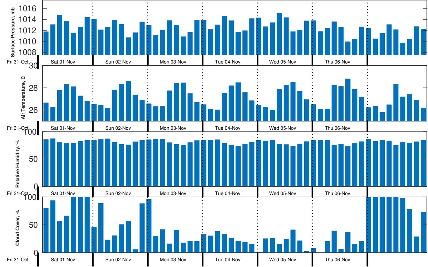
Met Forecast for CSA (ONHYM) PPL EBS - Liberia from 01-Nov-2025 00:00:00 to 08-Nov-2025 00:00:00
