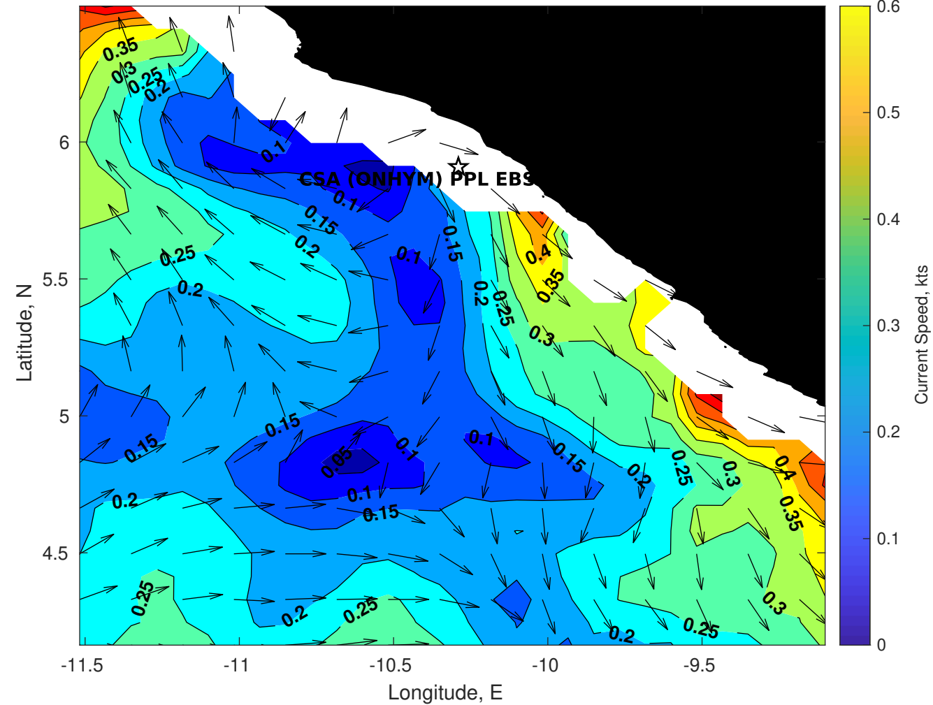
Surface Currents for CSA (ONHYM) PPL EBS - Liberia at 31-Oct-2025 00:00:00
