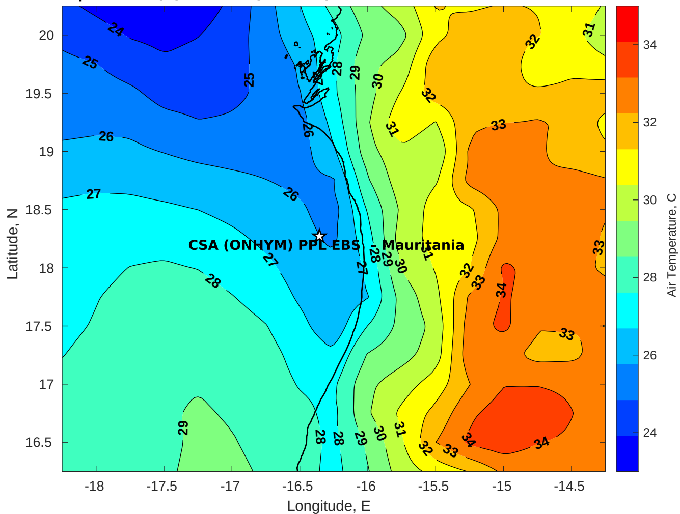
Air Temperature (C) for CSA (ONHYM) PPL EBS - Mauritania at 01-Nov-2025
