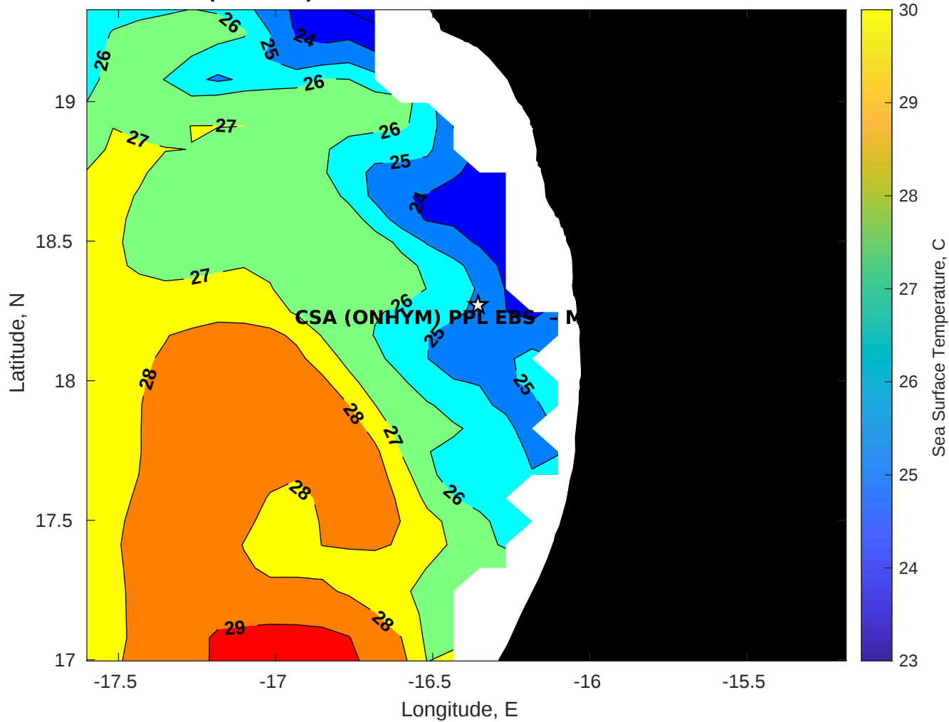
SST for CSA (ONHYM) PPL EBS - Mauritania at 31-Oct-2025 00:00:00
