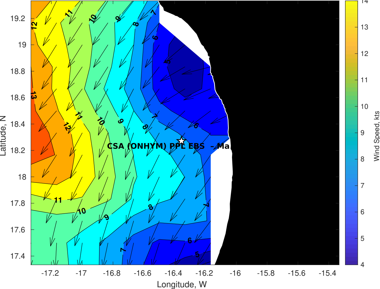
Winds (kts) for CSA (ONHYM) PPL EBS - Mauritania at 01-Nov-2025 09:00:00
