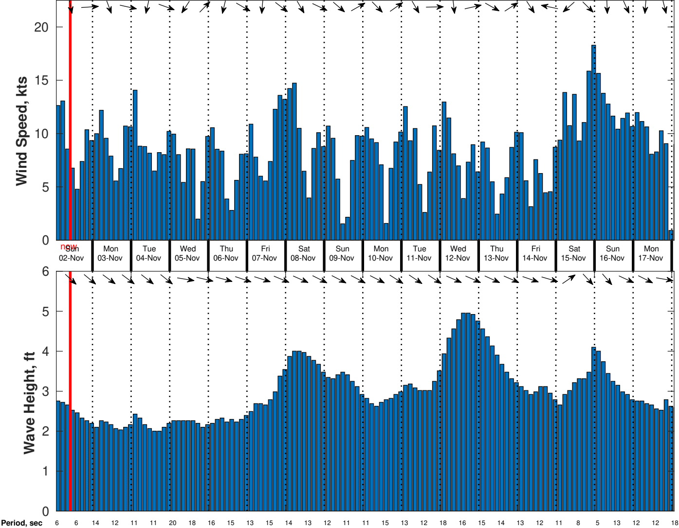
Wind & Wave Forecast for CSA (ONHYM) PPL EBS - Mauritania from 01-Nov-2025 01:00:00 to 17-Nov-2025 01:00:00
