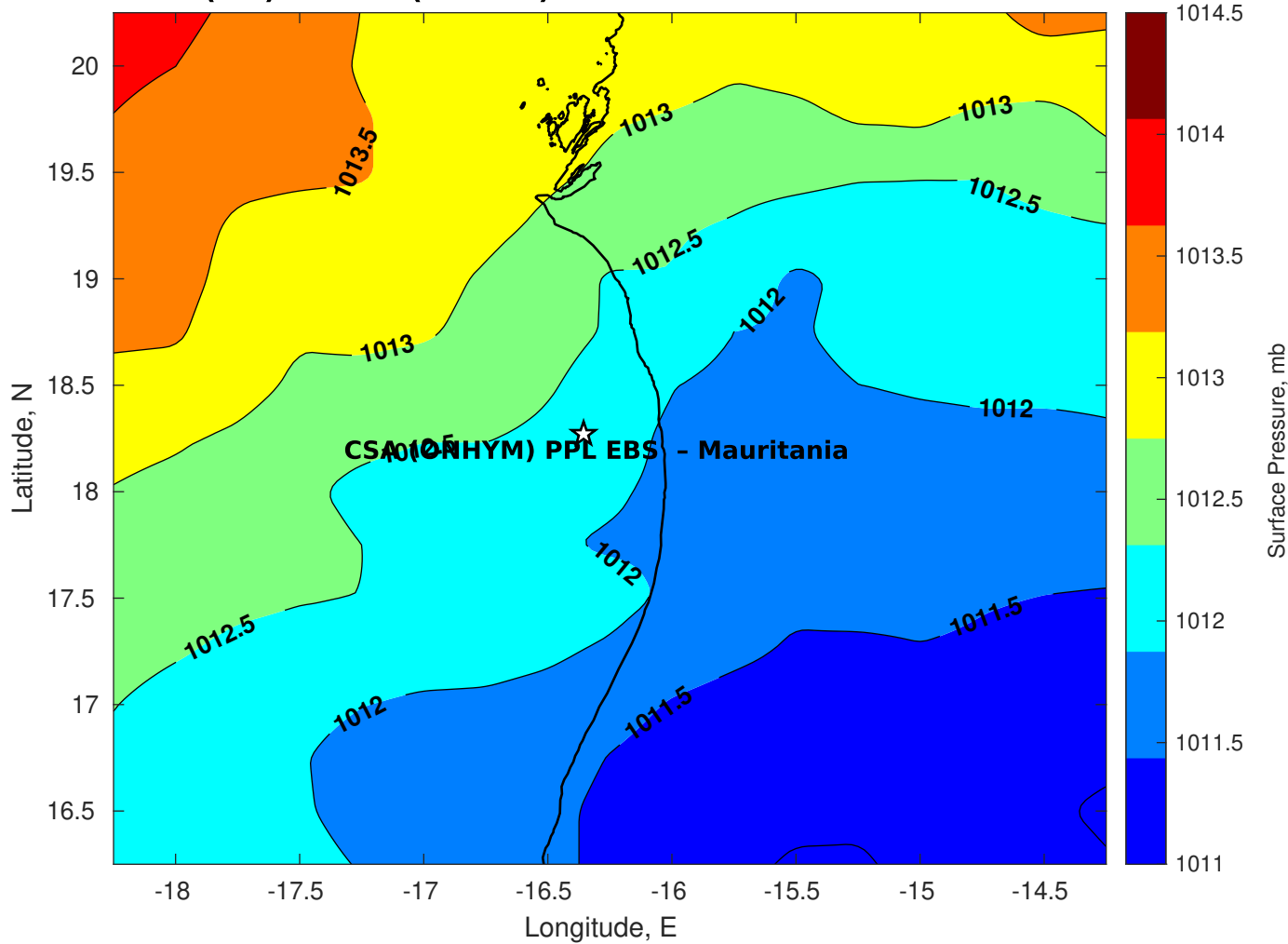
Surface Pressure (mb) for CSA (ONHYM) PPL EBS - Mauritania at 03-Nov-2025 00:00:00
