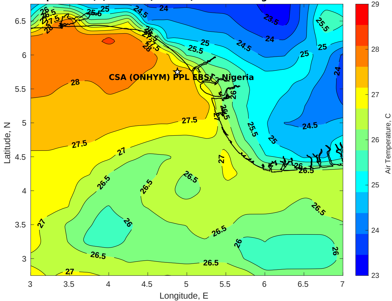
Air Temperature (C) for CSA (ONHYM) PPL EBS - Nigeria at 01-Nov-2025
