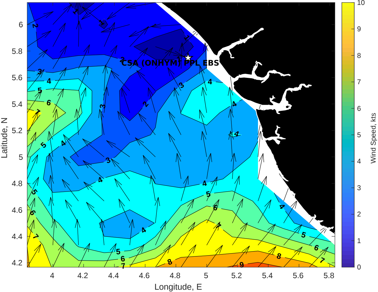
Winds (kts) for CSA (ONHYM) PPL EBS - Nigeria at 01-Nov-2025 09:00:00
