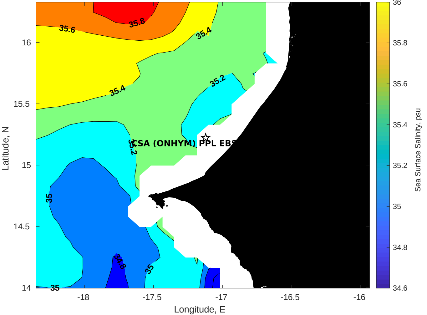
Surface Salinity for CSA (ONHYM) PPL EBS - Senegal at 31-Oct-2025 00:00:00
