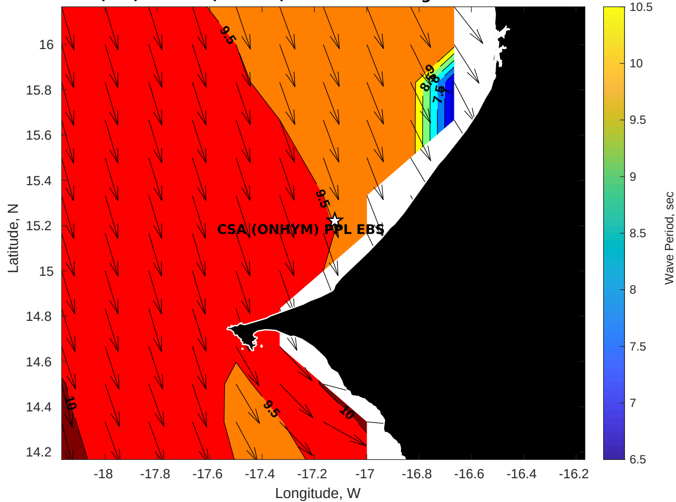
Wave Period (sec) for CSA (ONHYM) PPL EBS - Senegal at 01-Nov-2025 09:00:00
