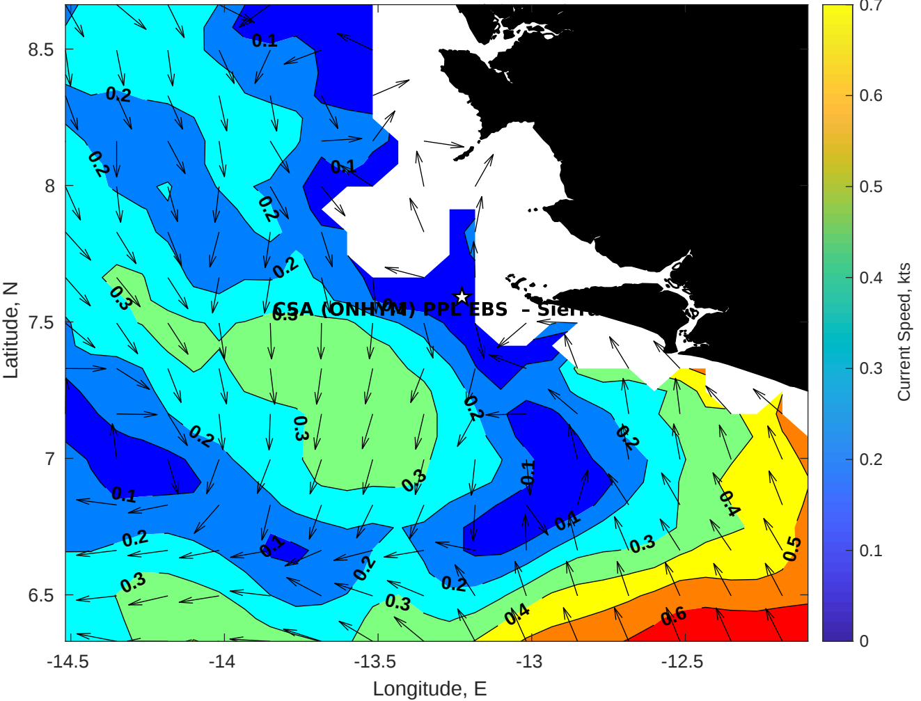
Surface Currents for CSA (ONHYM) PPL EBS - Sierra Leone at 31-Oct-2025 00:00:00
