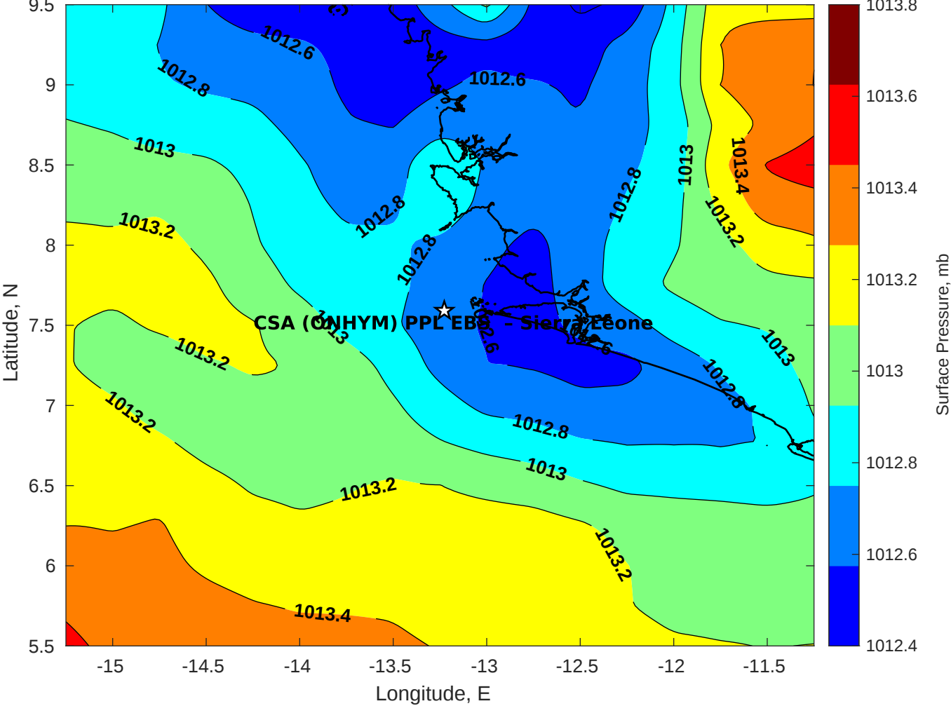
Surface Pressure (mb) for CSA (ONHYM) PPL EBS - Sierra Leone at 03-Nov-2025 00:00:00
