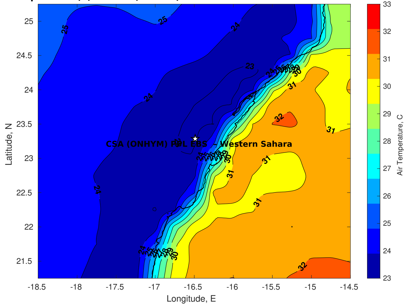
Air Temperature (C) for CSA (ONHYM) PPL EBS - Western Sahara at 01-Nov-2025
