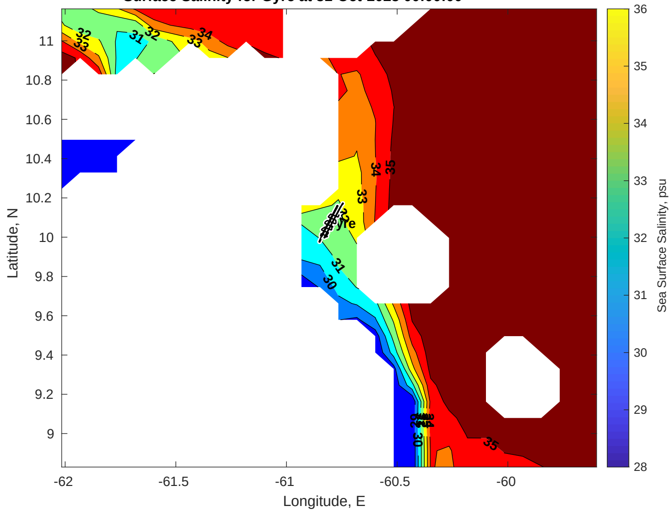
Surface Salinity for Gyre at 31-Oct-2025 00:00:00
