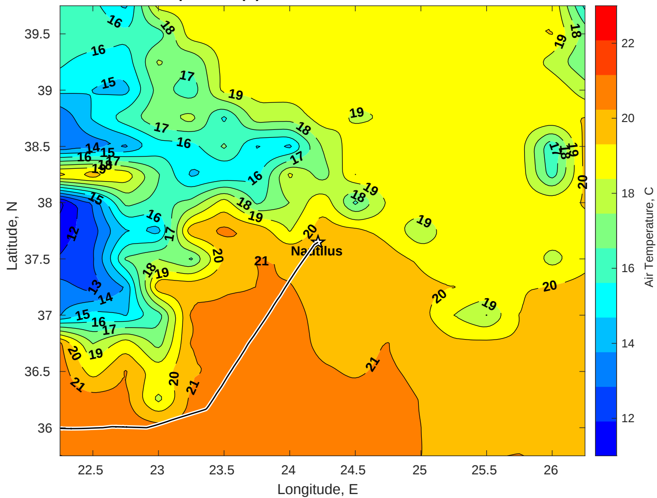
Air Temperature (C) for Nautilus at 01-Nov-2025
