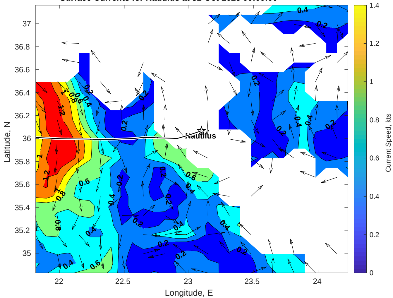
Surface Currents for Nautilus at 31-Oct-2025 00:00:00
