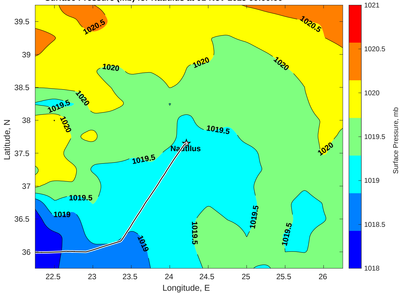
Surface Pressure (mb) for Nautilus at 01-Nov-2025 00:00:00
