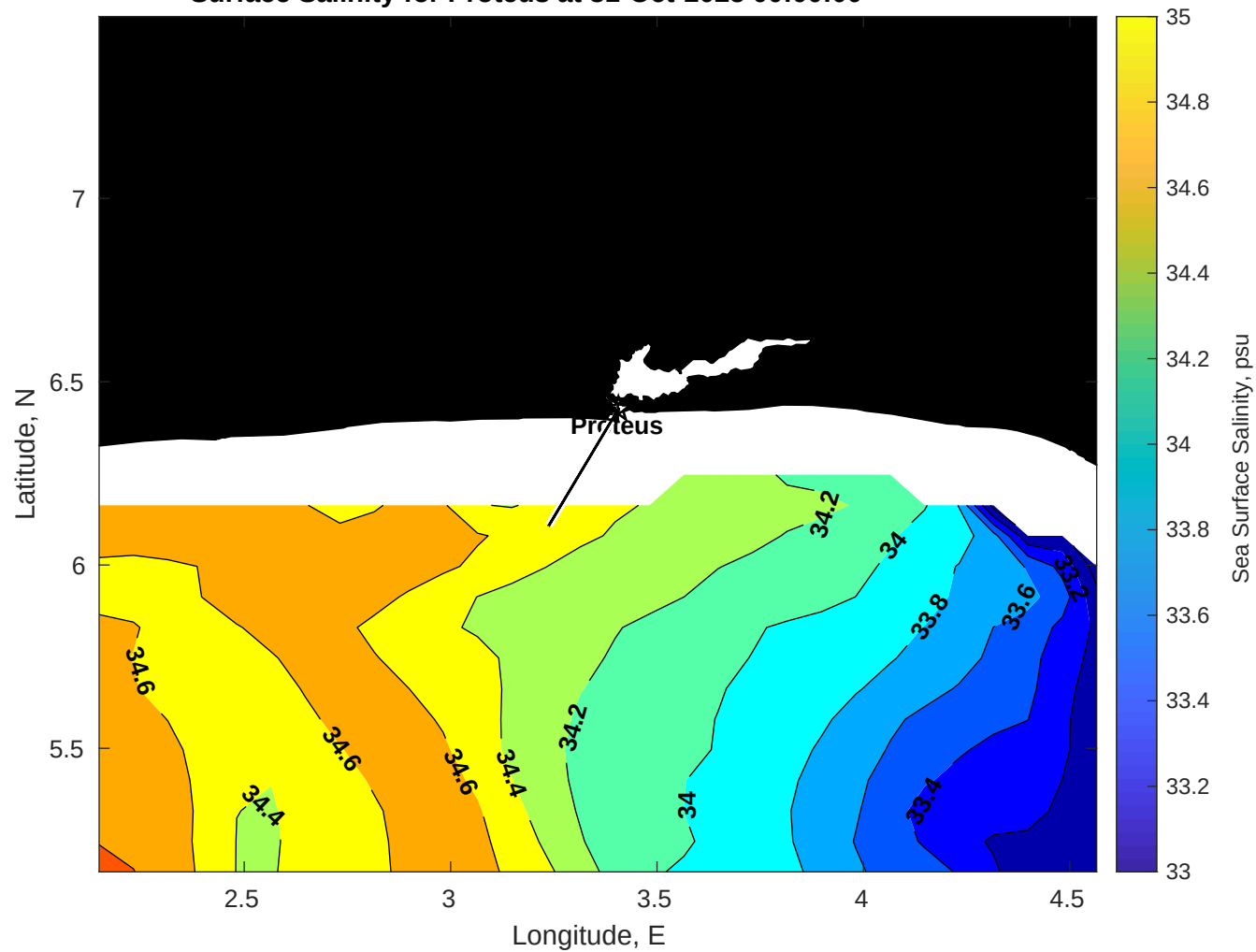
Surface Salinity for Proteus at 31-Oct-2025 00:00:00
