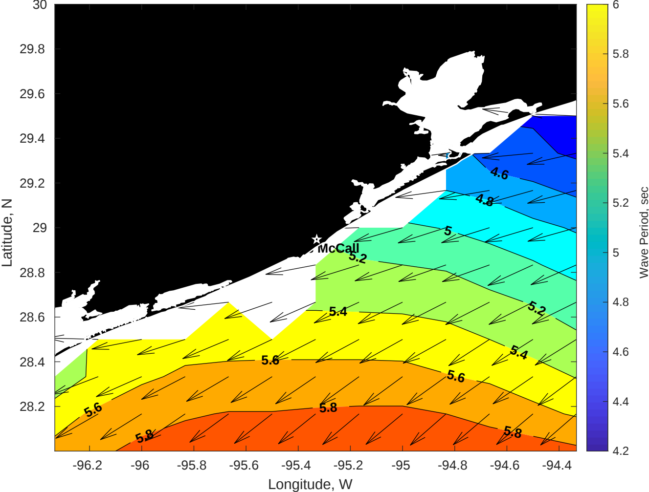
Wave Period (sec) for Brooks McCall at 02-Nov-2025 09:00:00
