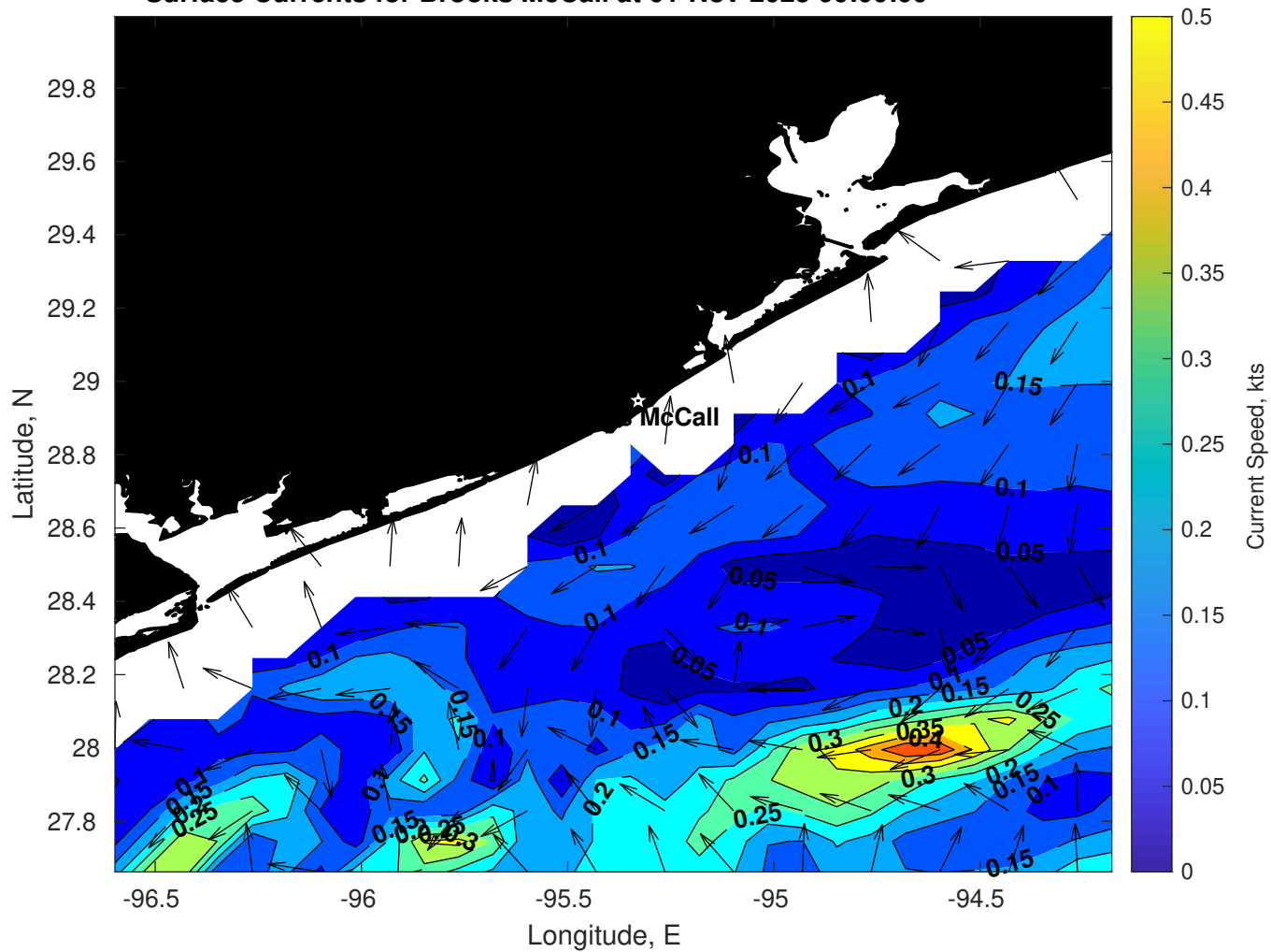
Surface Currents for Brooks McCall at 01-Nov-2025 00:00:00
