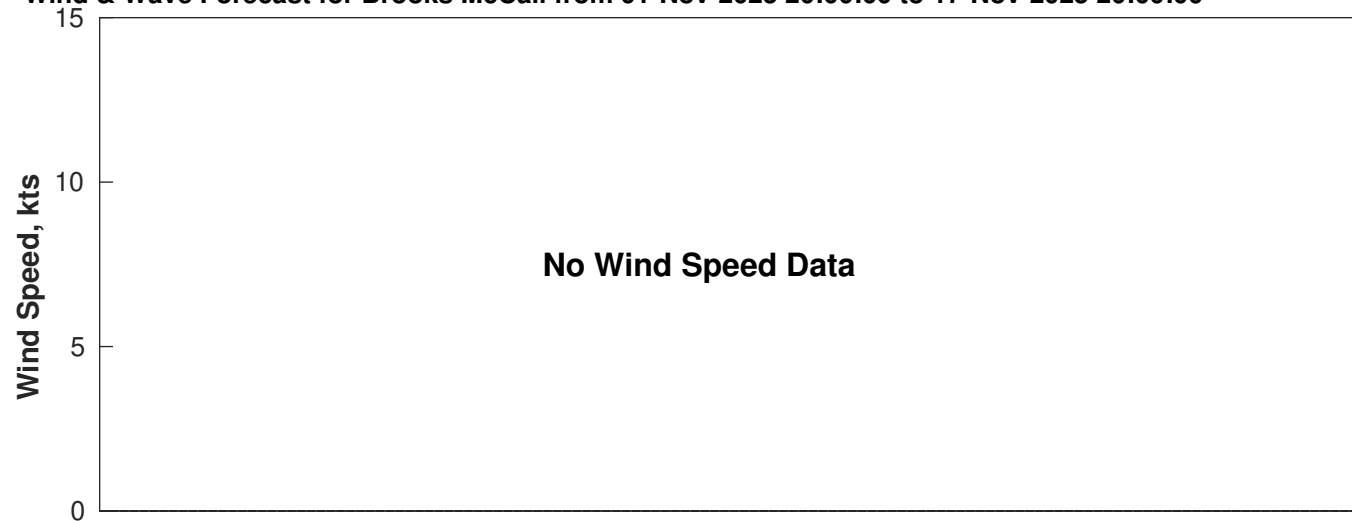
Wind & Wave Forecast for Brooks McCall from 01-Nov-2025 20:00:00 to 17-Nov-2025 20:00:00
