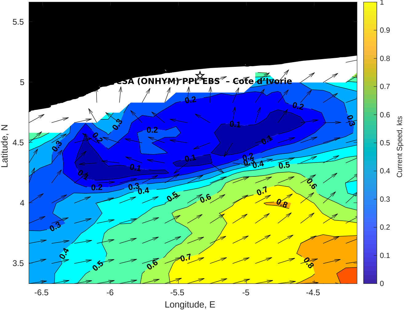
Surface Currents for CSA (ONHYM) PPL EBS - Cote d'Ivoire at 01-Nov-2025 00:00:00
