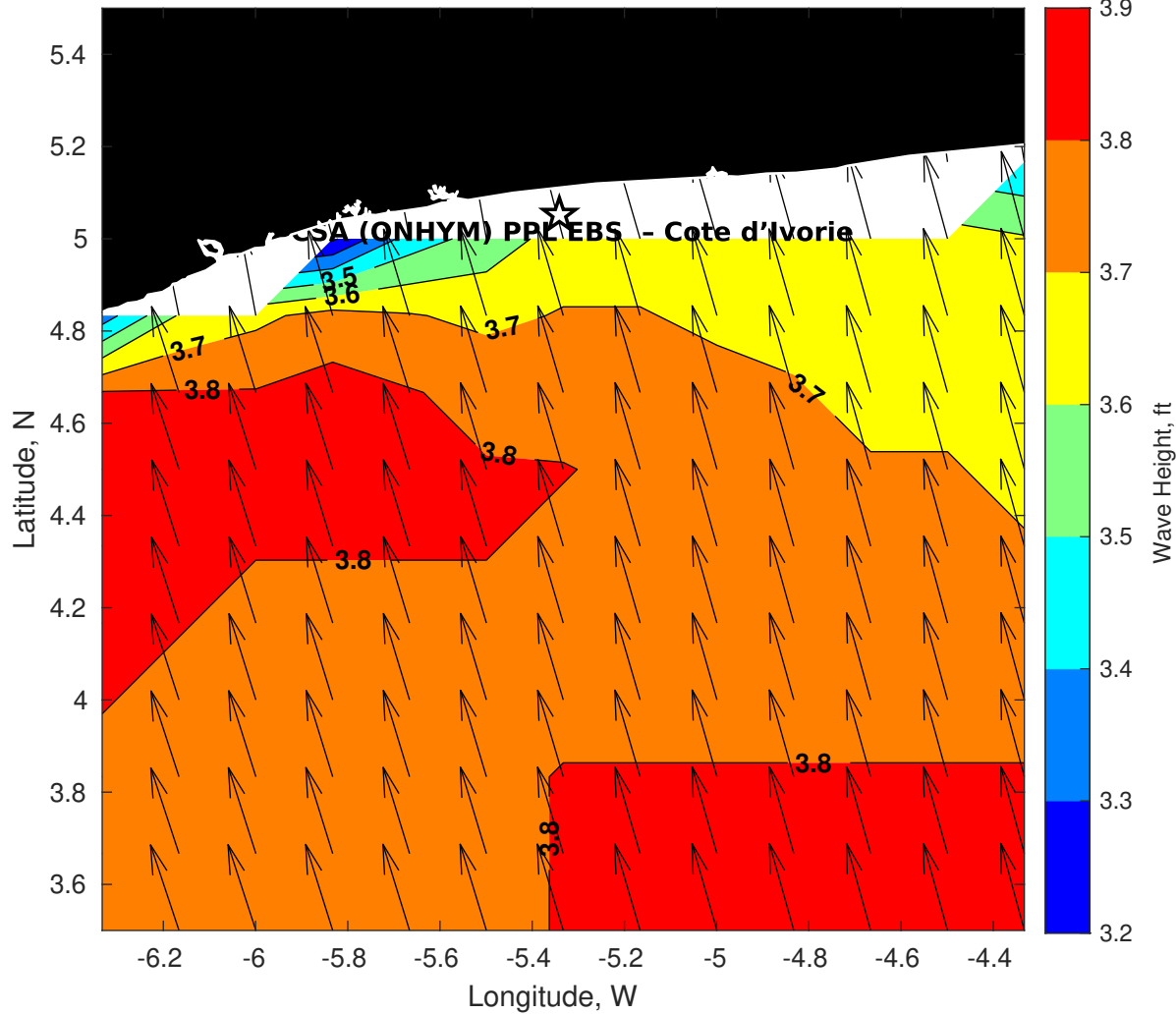
Wave Height (ft) for CSA (ONHYM) PPL EBS - Cote d'Ivoire at 02-Nov-2025 09:00:00
