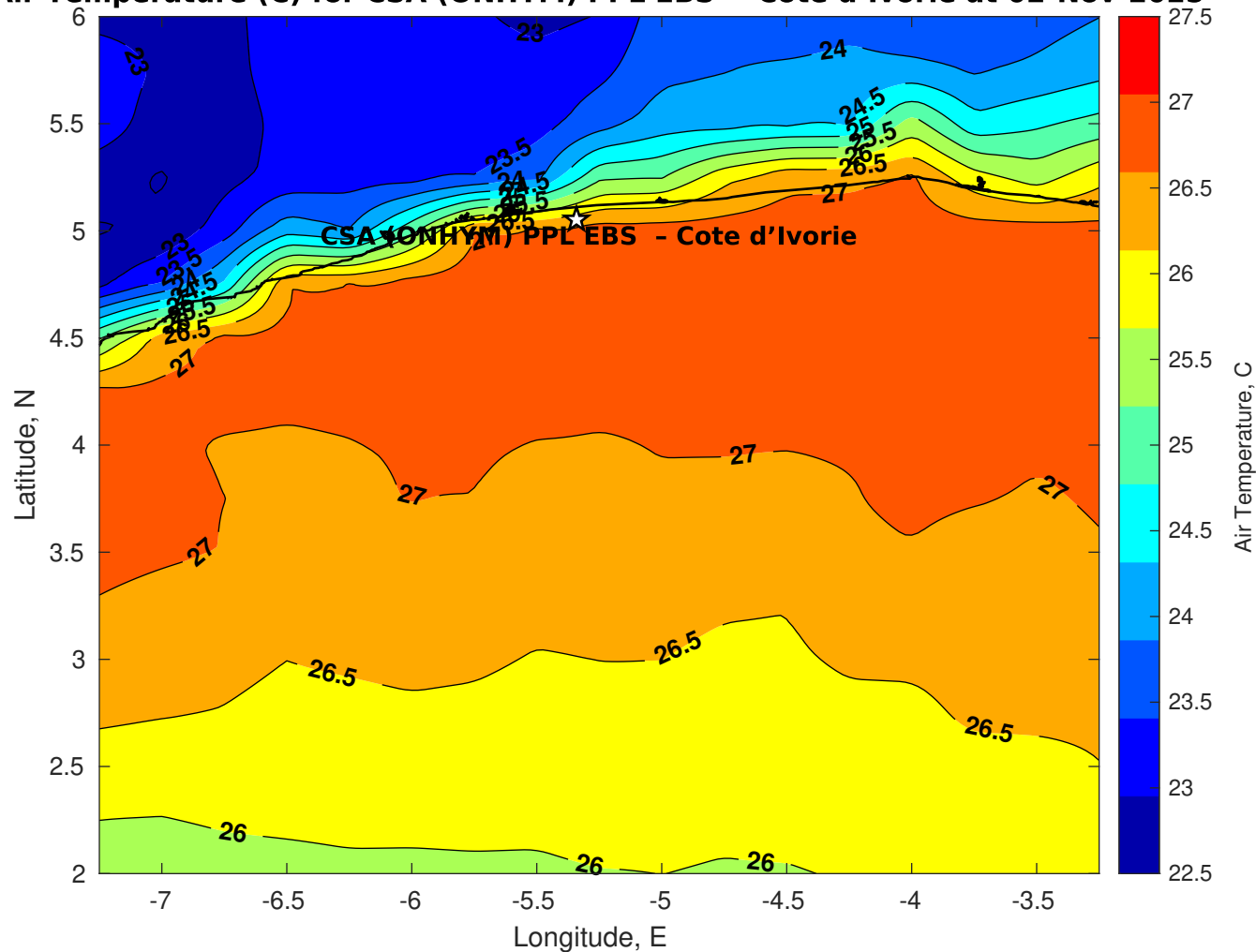
Air Temperature (C) for CSA (ONHYM) PPL EBS - Cote d'Ivoire at 02-Nov-2025
