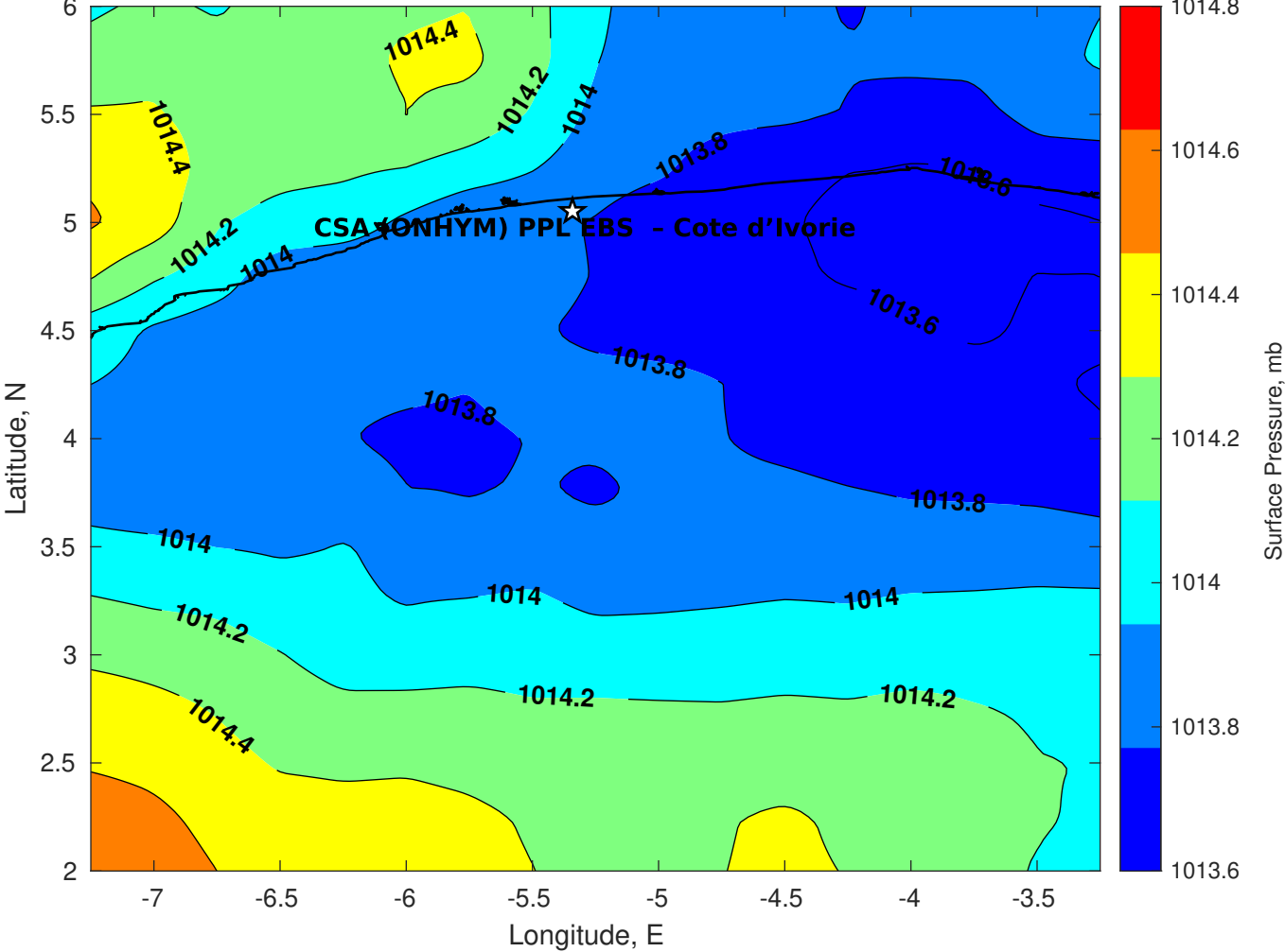
Surface Pressure (mb) for CSA (ONHYM) PPL EBS - Cote d'Ivoire at 04-Nov-2025 00:00:00
