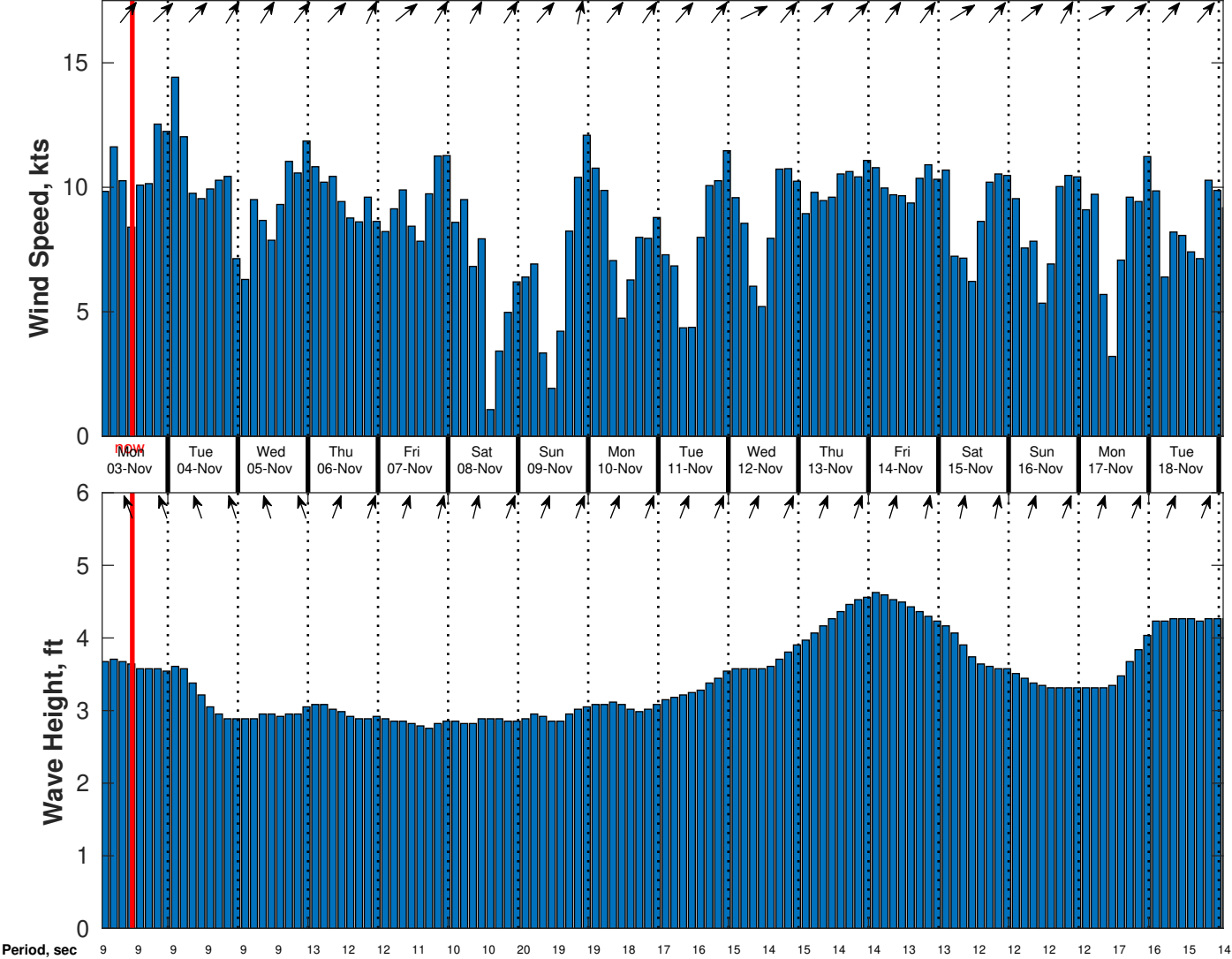
Wind & Wave Forecast for CSA (ONHYM) PPL EBS - Cote d'Ivoire from 02-Nov-2025 01:00:00 to 18-Nov-2025 01:00:00
