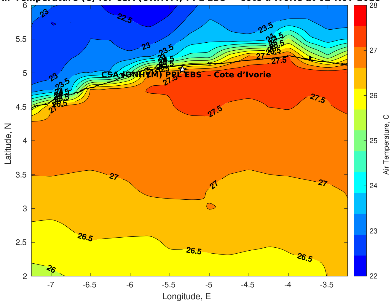
Air Temperature (C) for CSA (ONHYM) PPL EBS - Cote d'Ivoire at 02-Nov-2025
