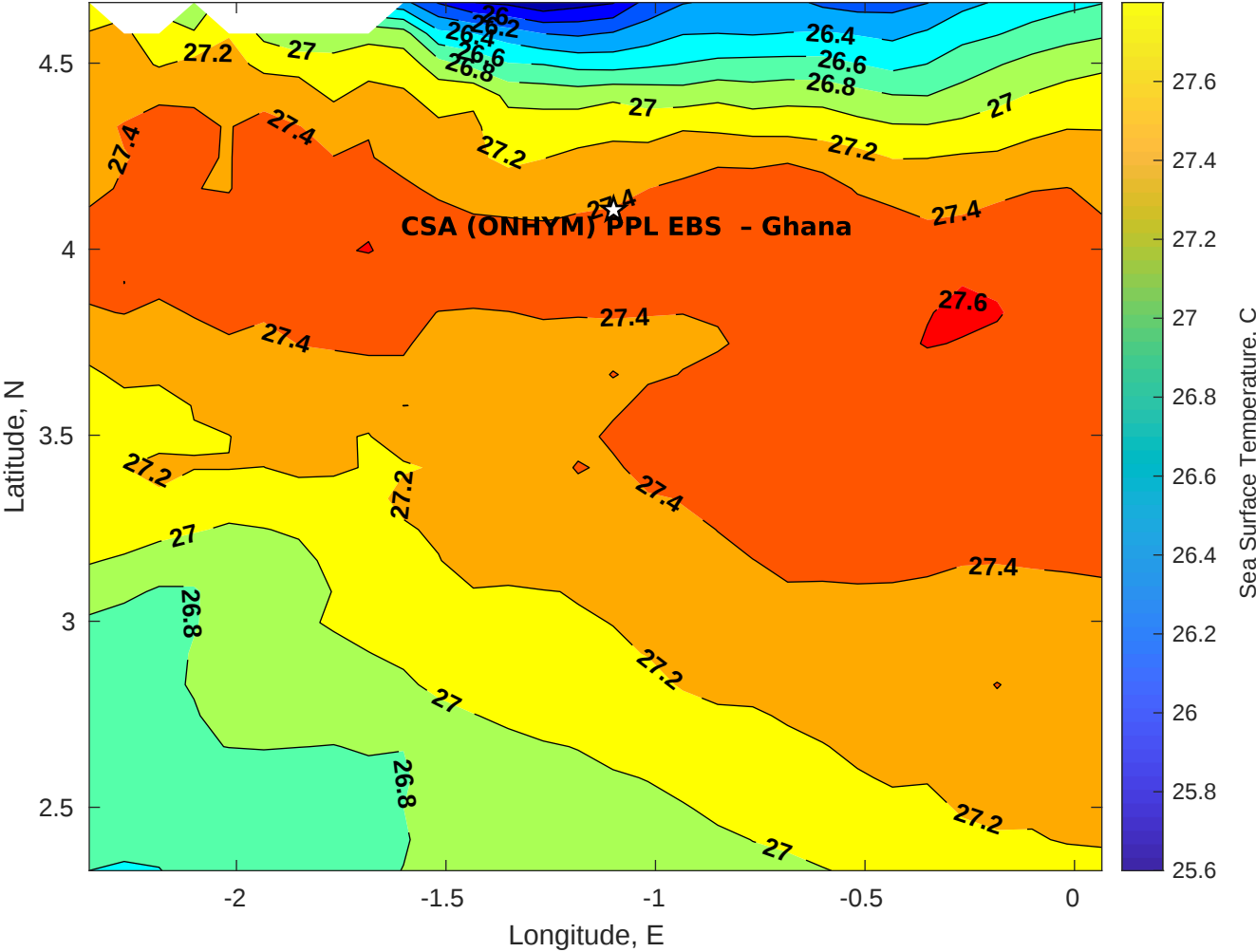
SST for CSA (ONHYM) PPL EBS - Ghana at 01-Nov-2025 00:00:00
