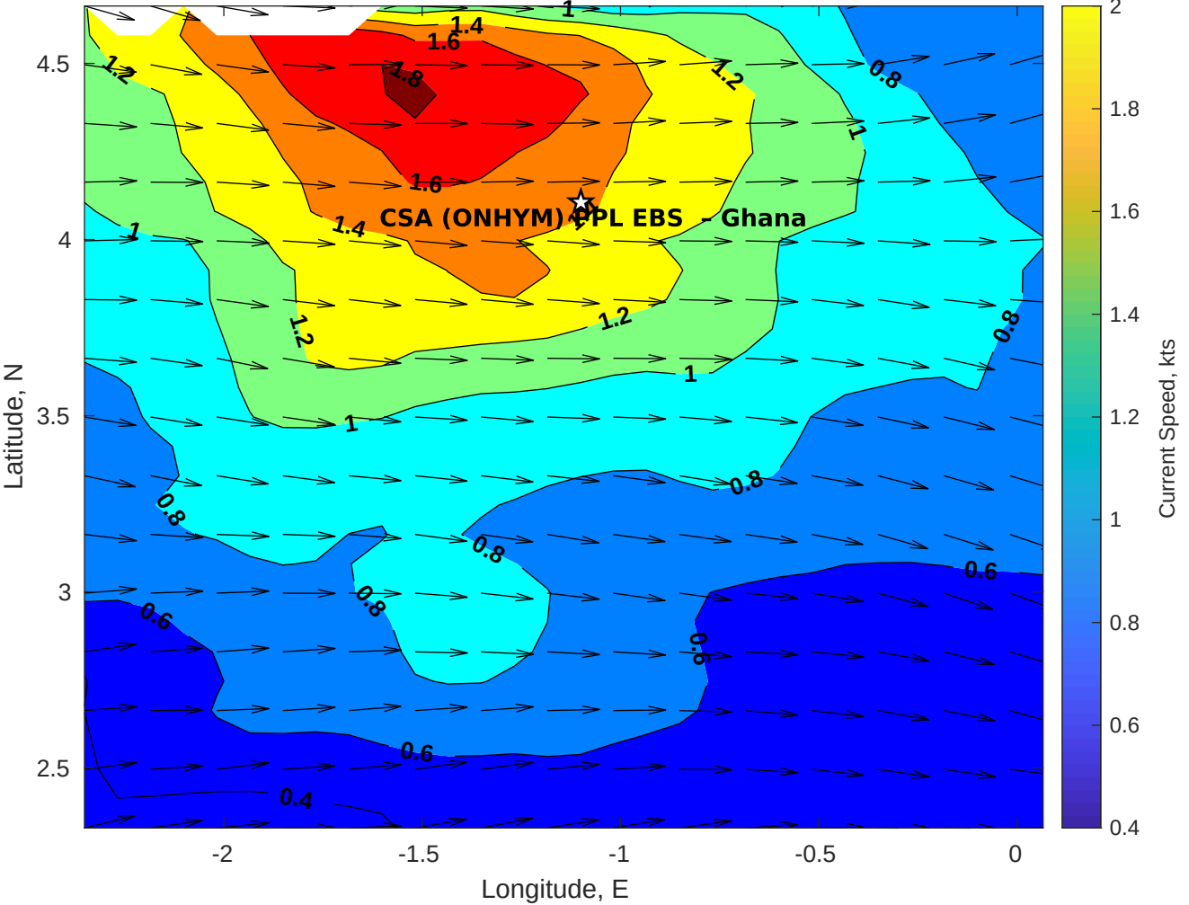
Surface Currents for CSA (ONHYM) PPL EBS - Ghana at 01-Nov-2025 00:00:00
