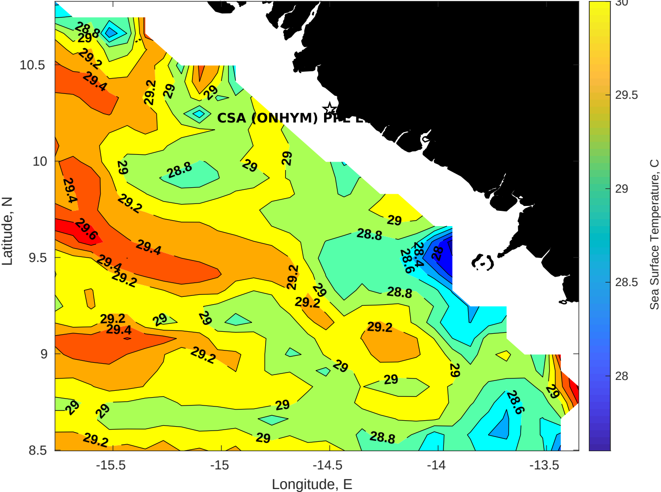
SST for CSA (ONHYM) PPL EBS - Guinea at 01-Nov-2025 00:00:00
