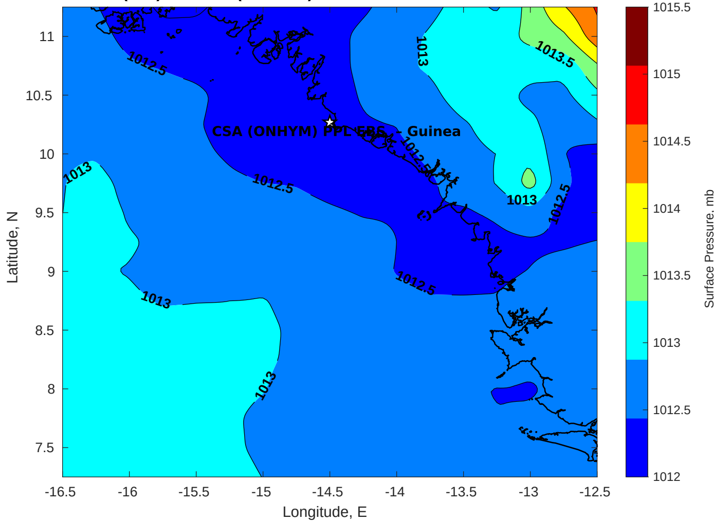
Surface Pressure (mb) for CSA (ONHYM) PPL EBS - Guinea at 03-Nov-2025 00:00:00
