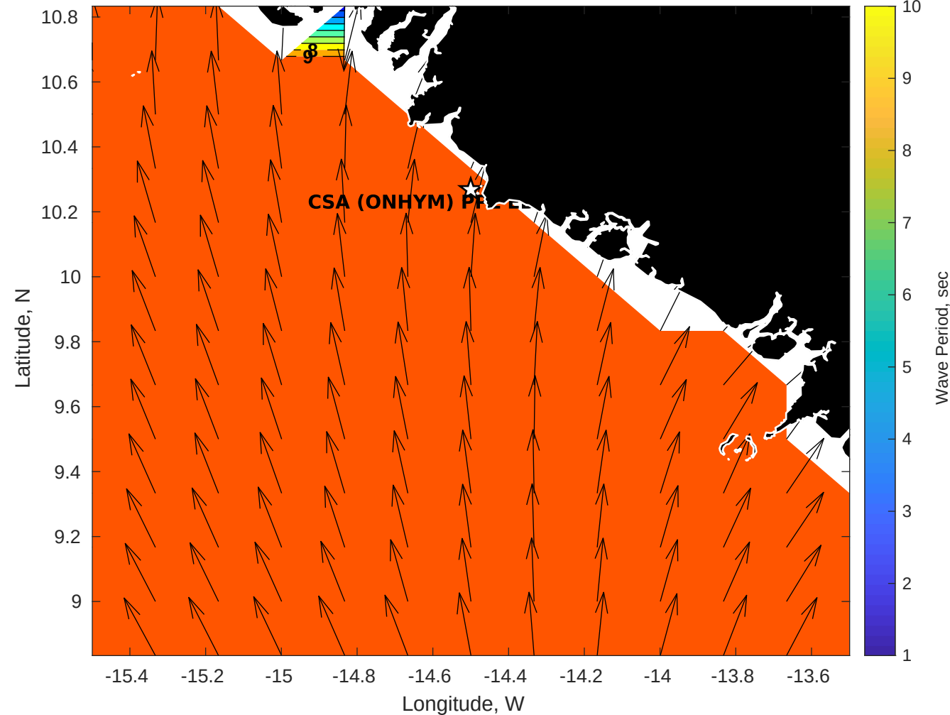
Wave Period (sec) for CSA (ONHYM) PPL EBS - Guinea at 02-Nov-2025 09:00:00
