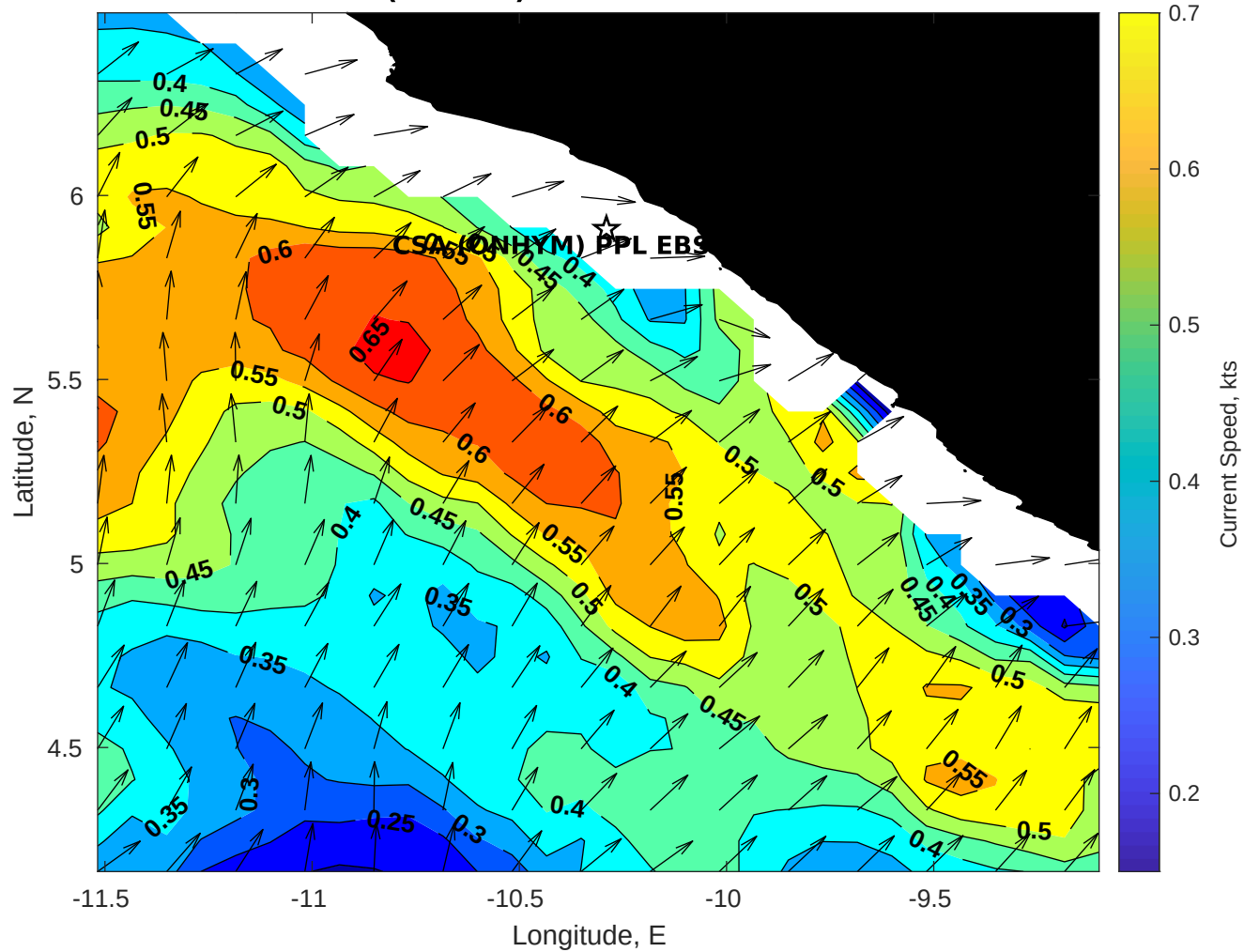
Surface Currents for CSA (ONHYM) PPL EBS - Liberia at 01-Nov-2025 00:00:00
