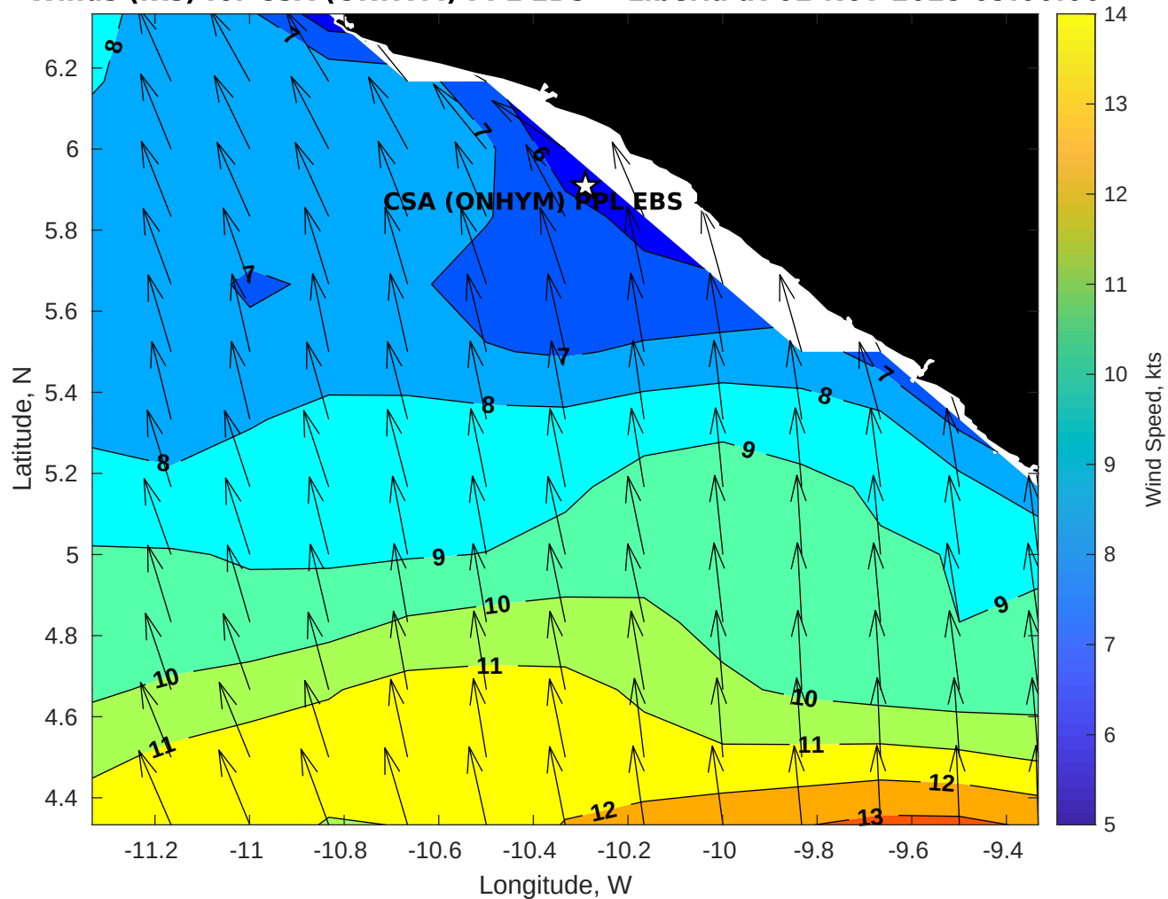
Winds (kts) for CSA (ONHYM) PPL EBS - Liberia at 02-Nov-2025 09:00:00
