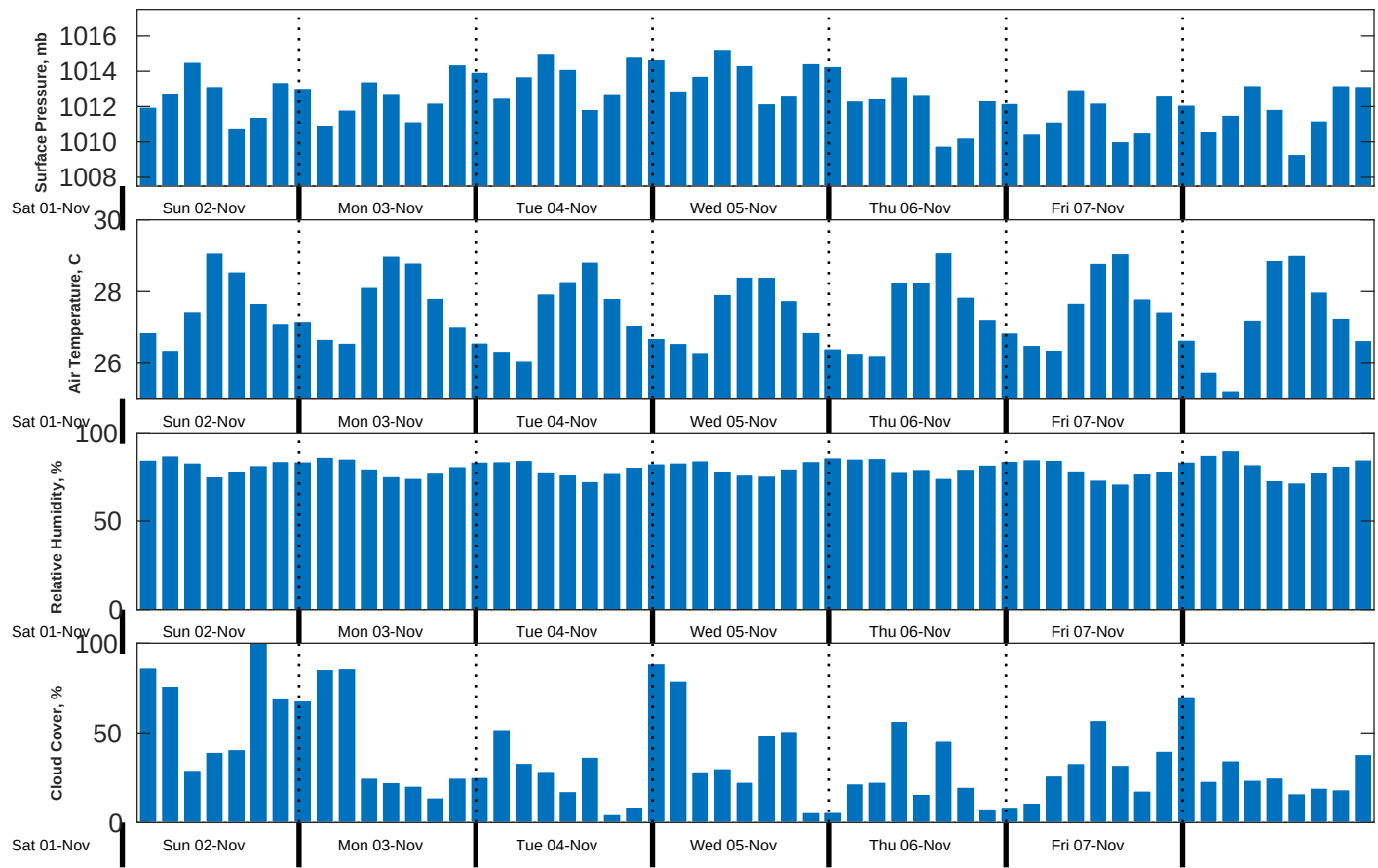
Met Forecast for CSA (ONHYM) PPL EBS - Liberia from 02-Nov-2025 00:00:00 to 09-Nov-2025 00:00:00
