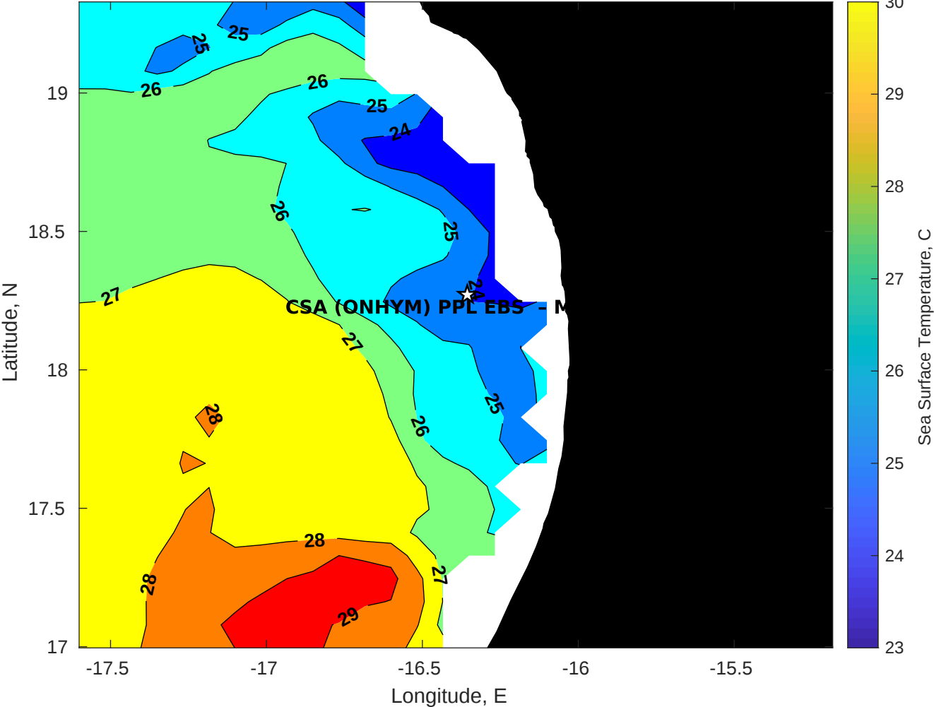
SST for CSA (ONHYM) PPL EBS - Mauritania at 01-Nov-2025 00:00:00
