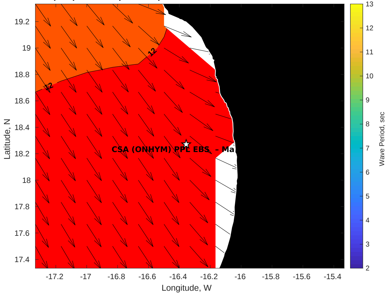
Wave Period (sec) for CSA (ONHYM) PPL EBS - Mauritania at 02-Nov-2025 09:00:00
