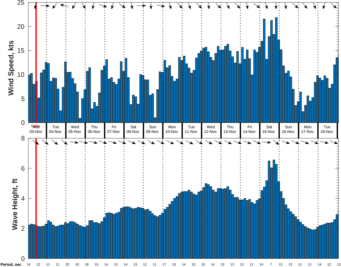
Wind & Wave Forecast for CSA (ONHYM) PPL EBS - Mauritania from 02-Nov-2025 01:00:00 to 18-Nov-2025 01:00:00
