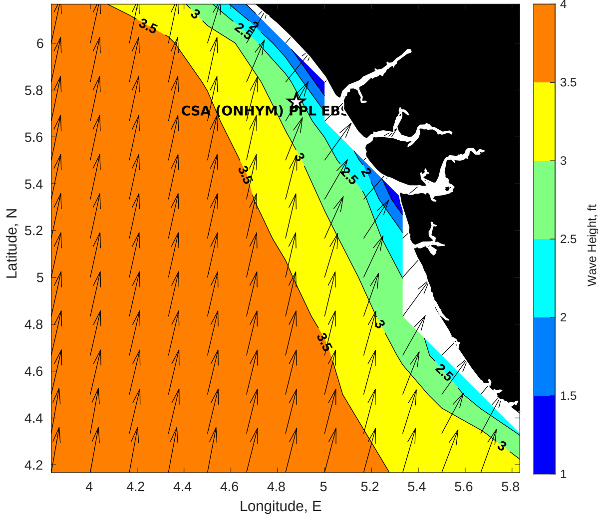
Wave Height (ft) for CSA (ONHYM) PPL EBS - Nigeria at 02-Nov-2025 09:00:00
