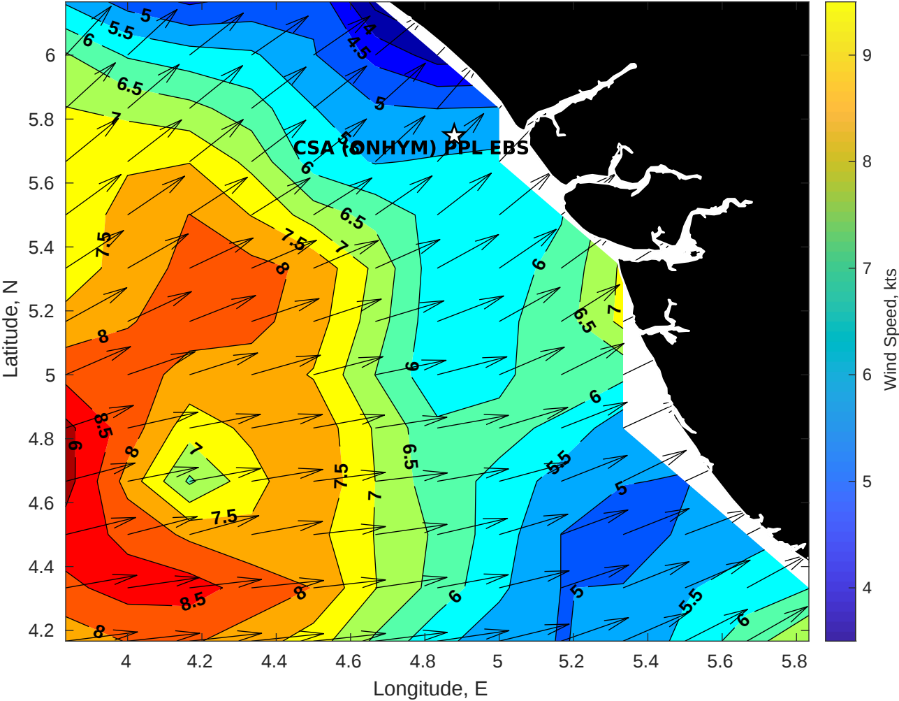
Winds (kts) for CSA (ONHYM) PPL EBS - Nigeria at 02-Nov-2025 09:00:00
