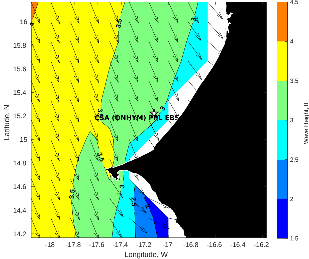
Wave Height (ft) for CSA (ONHYM) PPL EBS - Senegal at 02-Nov-2025 09:00:00
