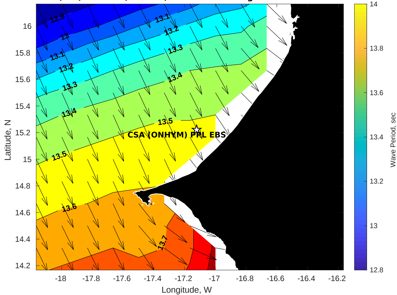
Wave Period (sec) for CSA (ONHYM) PPL EBS - Senegal at 02-Nov-2025 09:00:00
