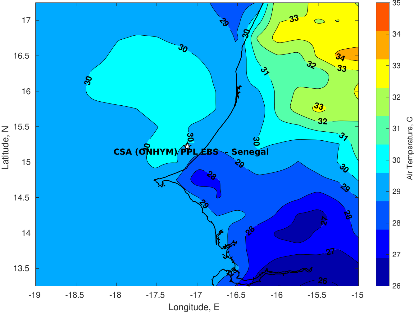
Air Temperature (C) for CSA (ONHYM) PPL EBS - Senegal at 02-Nov-2025
