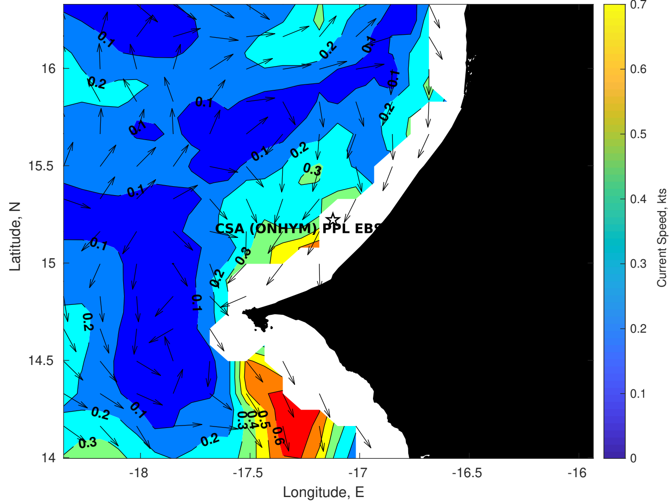
Surface Currents for CSA (ONHYM) PPL EBS - Senegal at 01-Nov-2025 00:00:00
