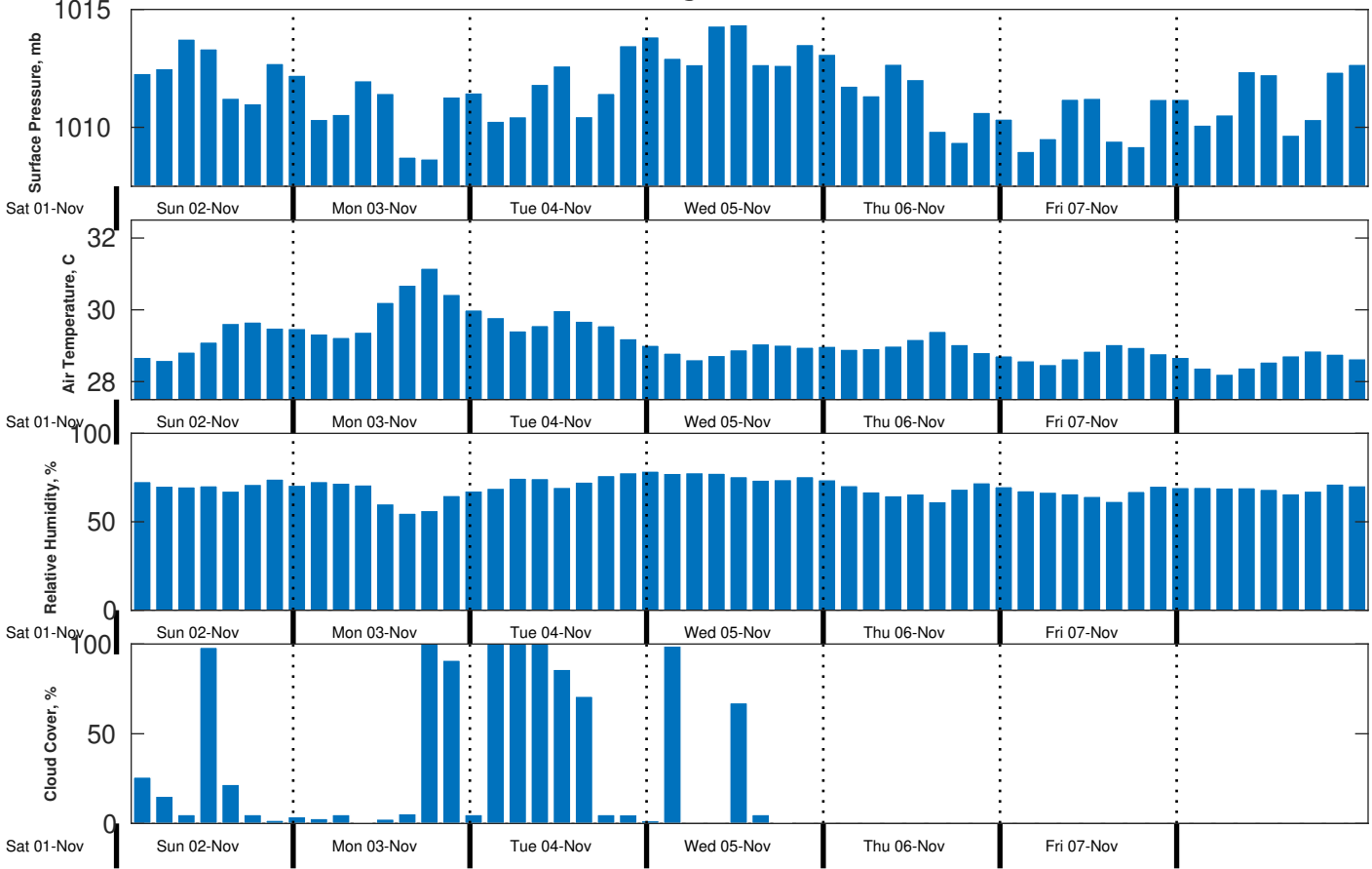
Met Forecast for CSA (ONHYM) PPL EBS - Senegal from 02-Nov-2025 00:00:00 to 09-Nov-2025 00:00:00
