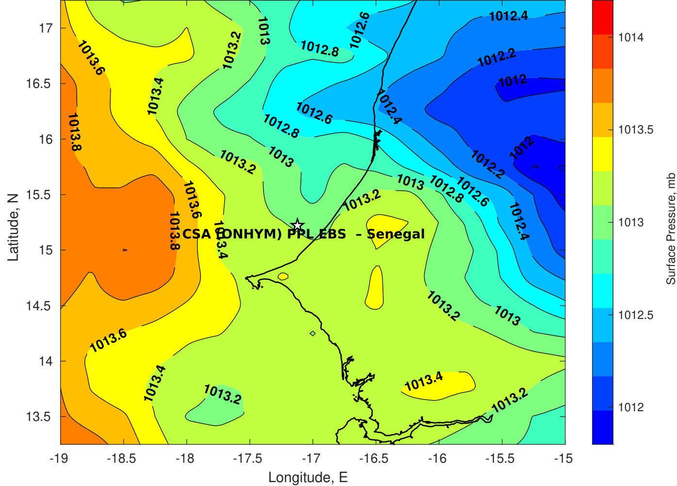
Surface Pressure (mb) for CSA (ONHYM) PPL EBS - Senegal at 02-Nov-2025 00:00:00
