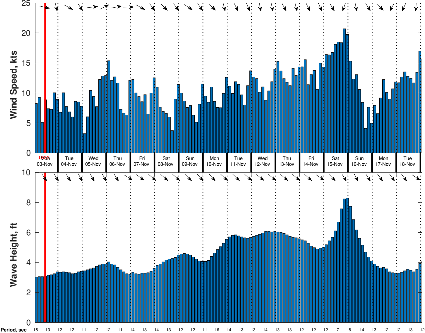
Wind & Wave Forecast for CSA (ONHYM) PPL EBS - Senegal from 02-Nov-2025 01:00:00 to 18-Nov-2025 01:00:00
