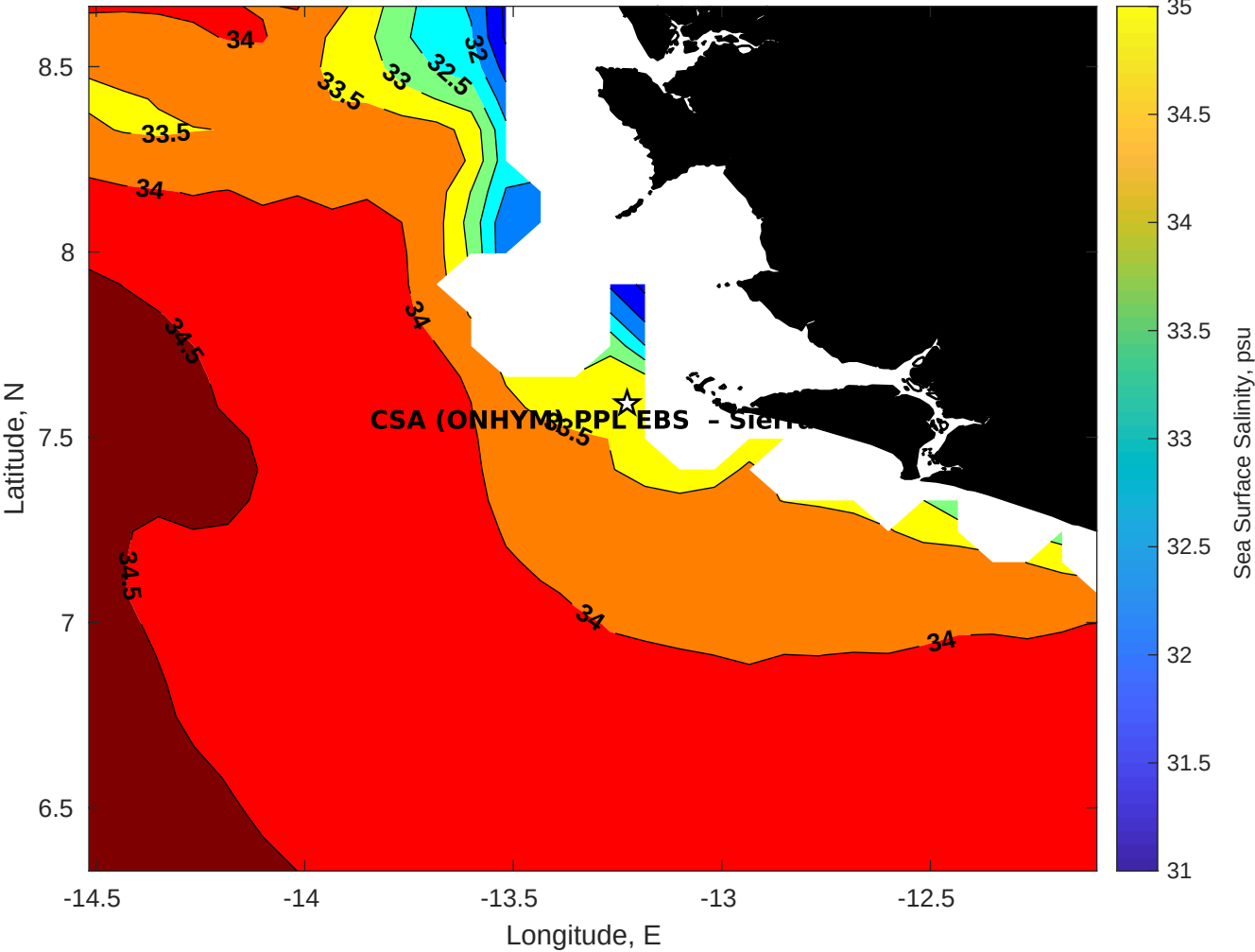
Surface Salinity for CSA (ONHYM) PPL EBS - Sierra Leone at 01-Nov-2025 00:00:00
