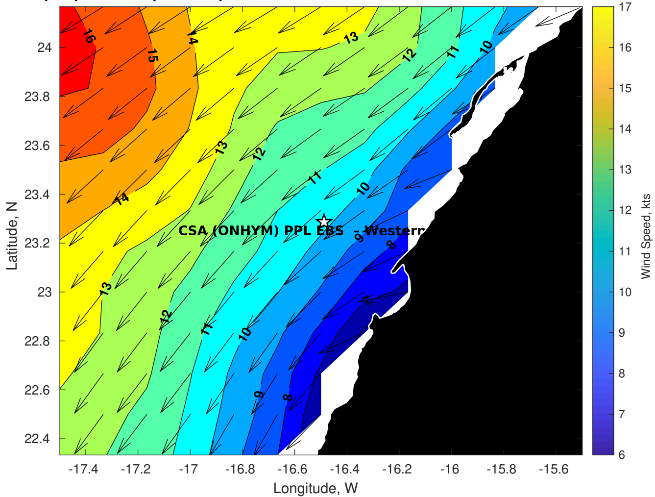
Winds (kts) for CSA (ONHYM) PPL EBS - Western Sahara at 02-Nov-2025 09:00:00
