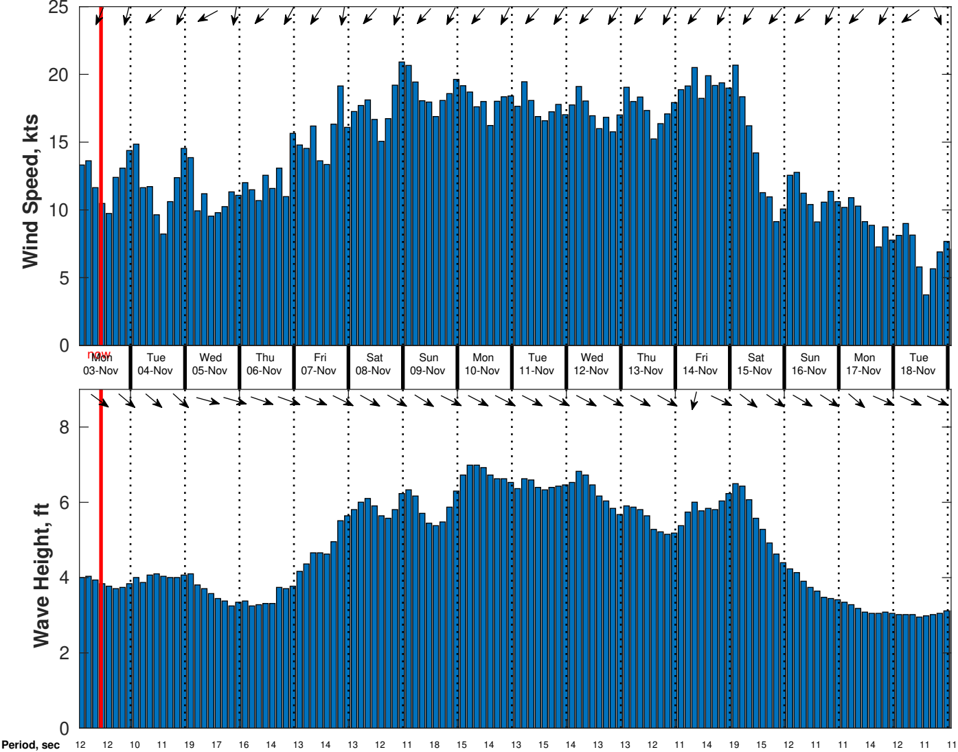
Wind & Wave Forecast for CSA (ONHYM) PPL EBS - Western Sahara from 02-Nov-2025 01:00:00 to 18-Nov-2025 01:00:00
