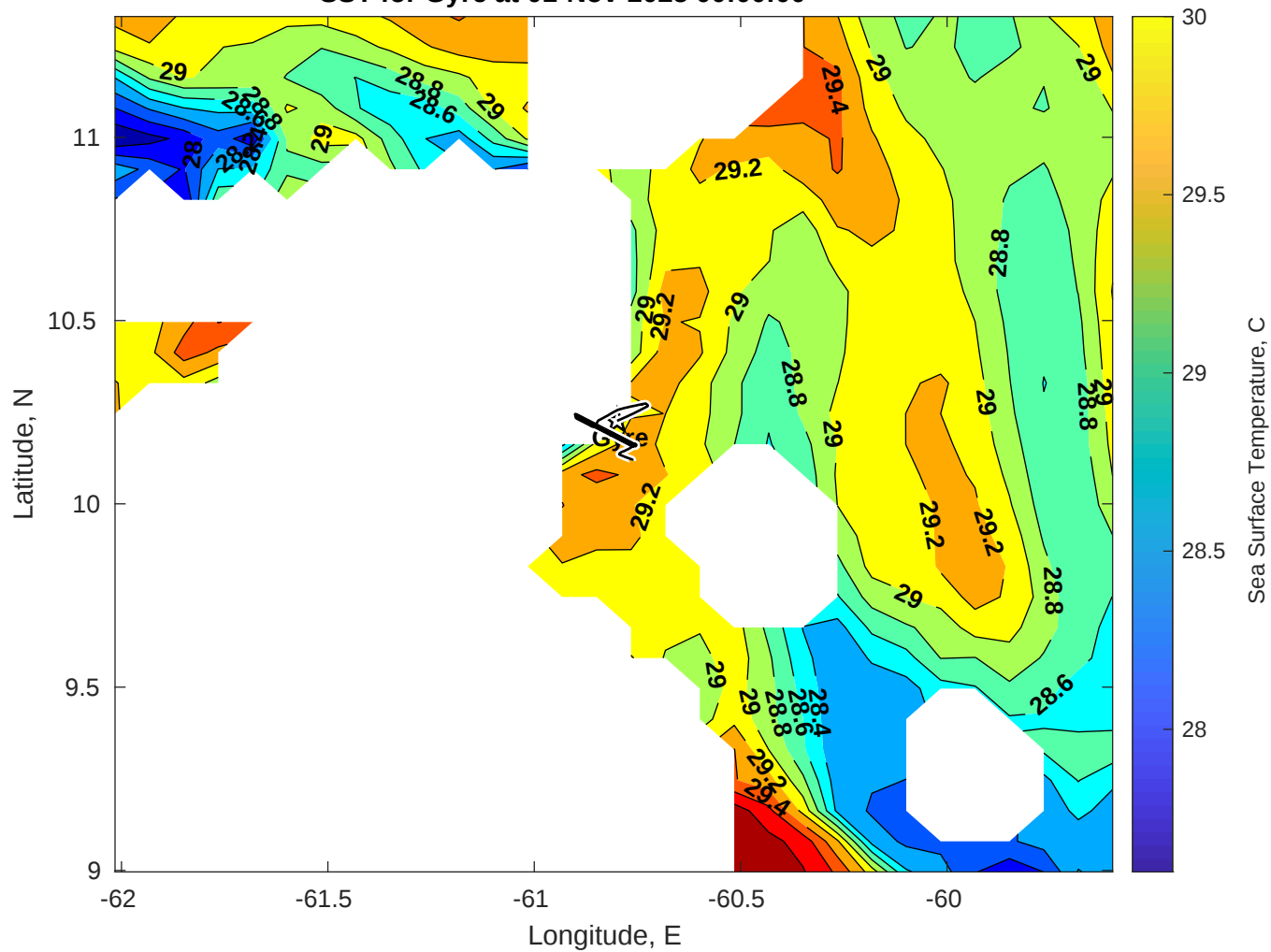
SST for Gyre at 01-Nov-2025 00:00:00
