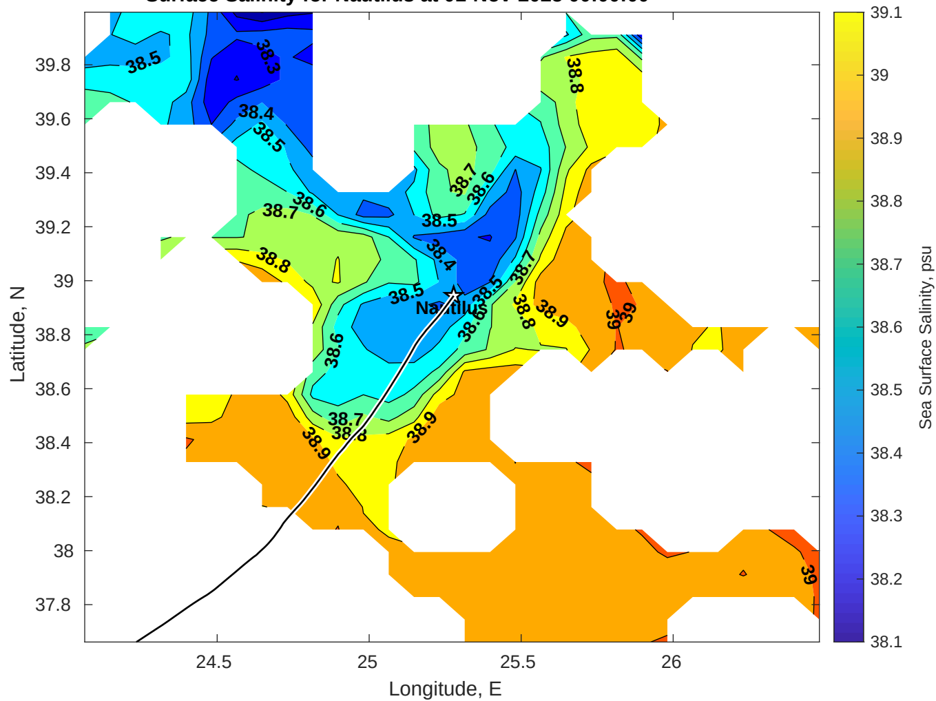
Surface Salinity for Nautilus at 01-Nov-2025 00:00:00
