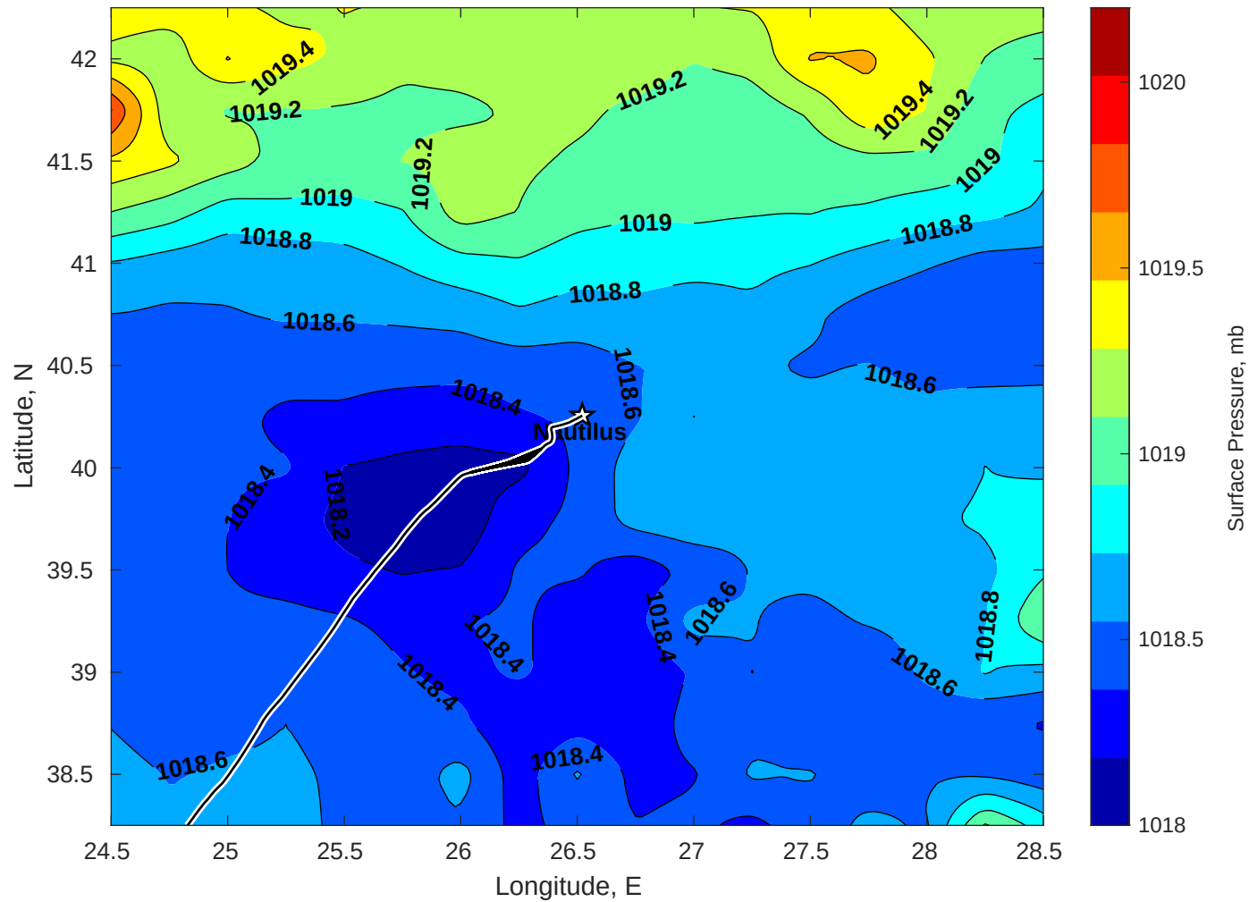
Surface Pressure (mb) for Nautilus at 03-Nov-2025 00:00:00
