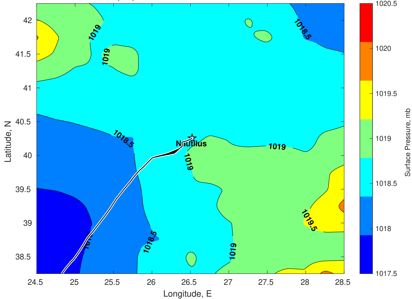
Surface Pressure (mb) for Nautilus at 04-Nov-2025 00:00:00
