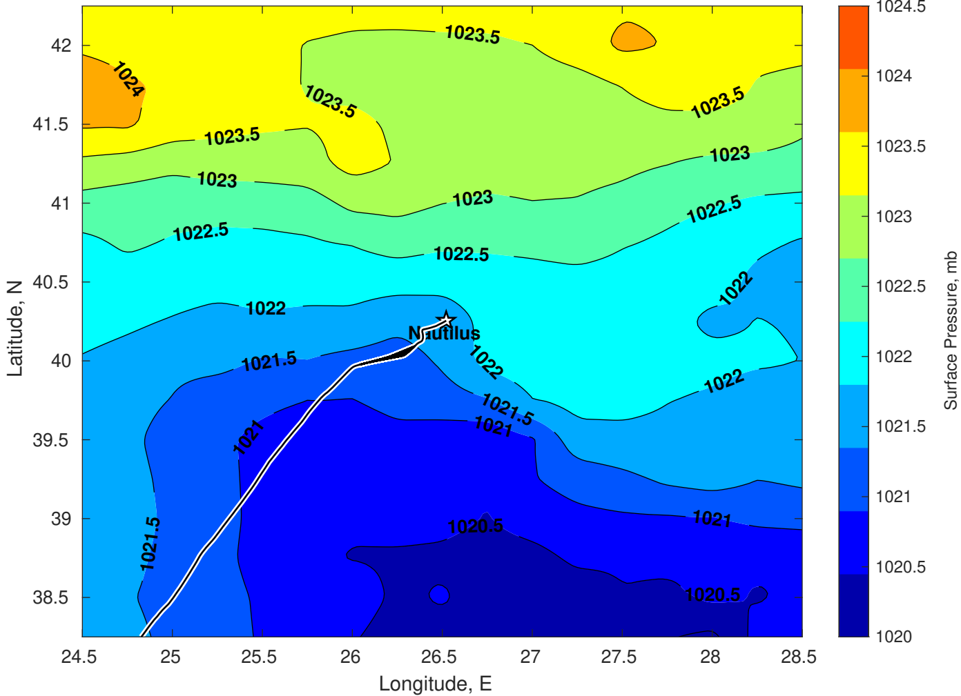
Surface Pressure (mb) for Nautilus at 02-Nov-2025 00:00:00
