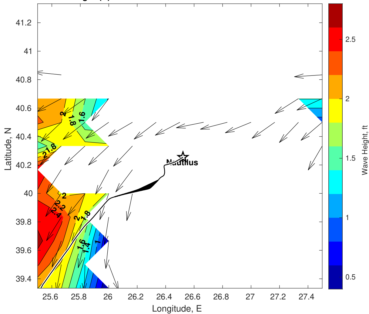
Wave Height (ft) for Nautilus at 02-Nov-2025 09:00:00
