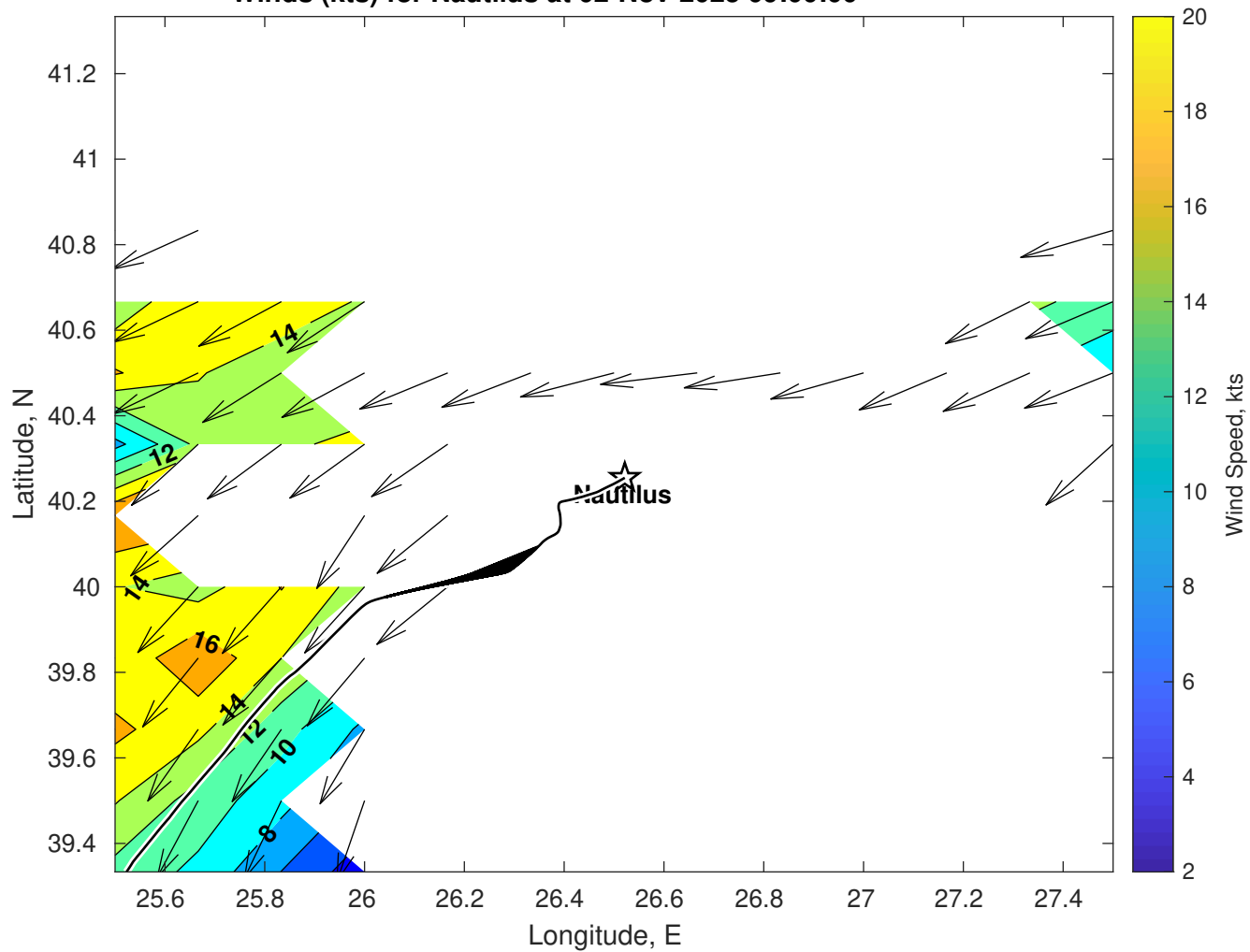
Winds (kts) for Nautilus at 02-Nov-2025 09:00:00
