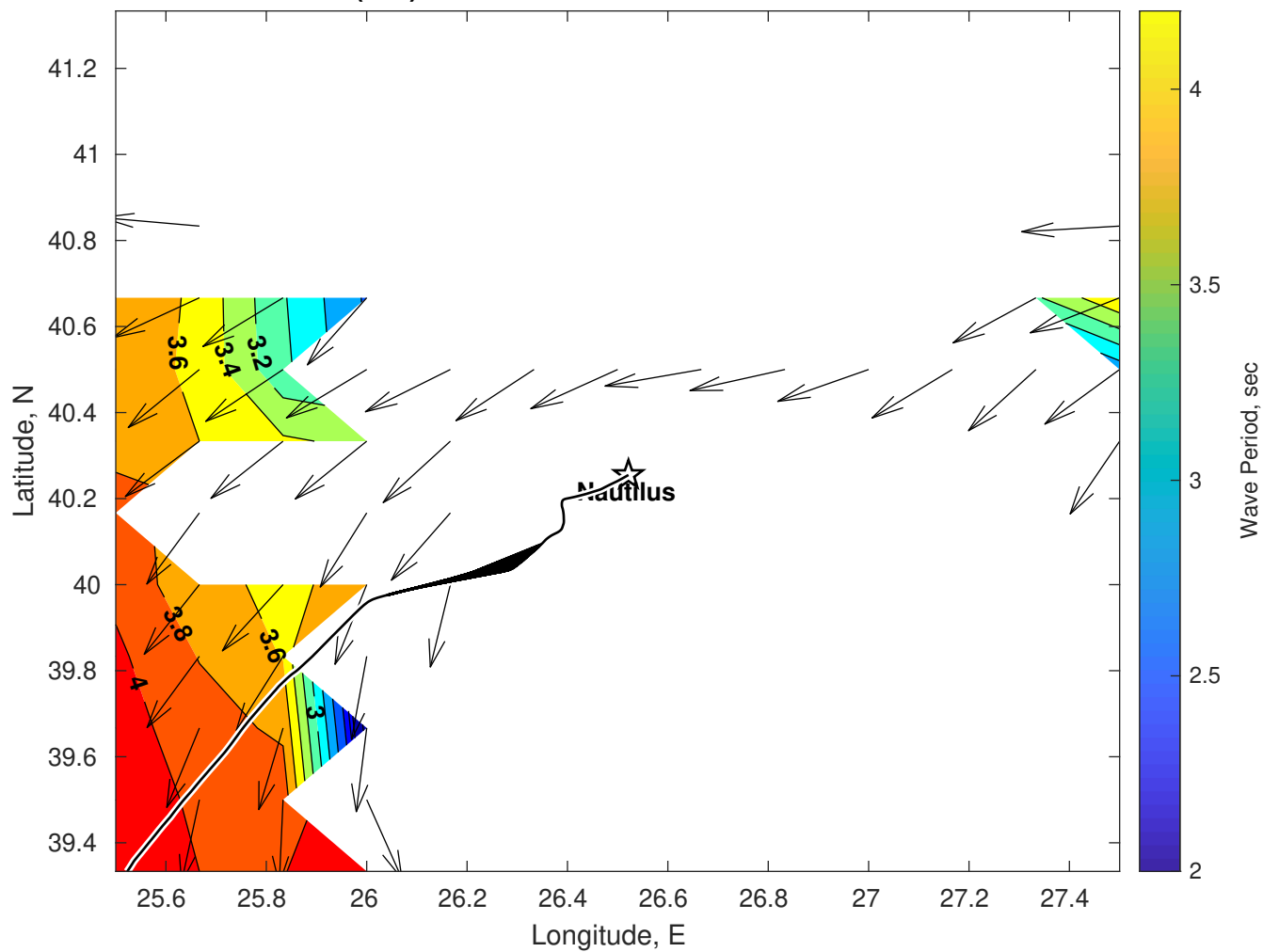
Wave Period (sec) for Nautilus at 02-Nov-2025 09:00:00
