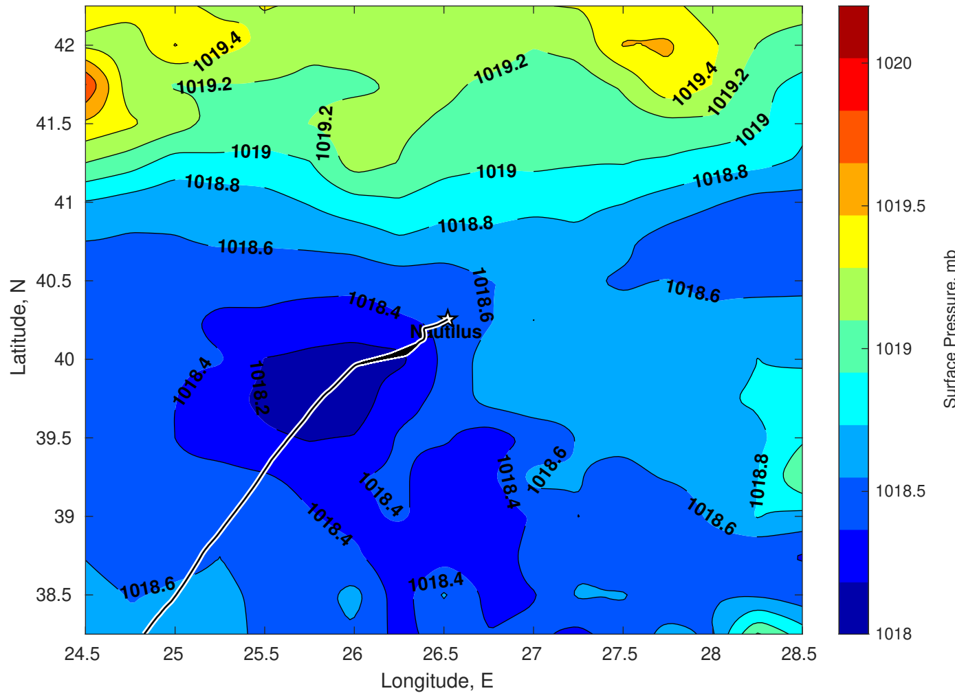
Surface Pressure (mb) for Nautilus at 03-Nov-2025 00:00:00
