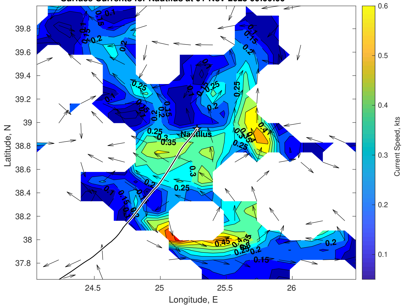
Surface Currents for Nautilus at 01-Nov-2025 00:00:00
