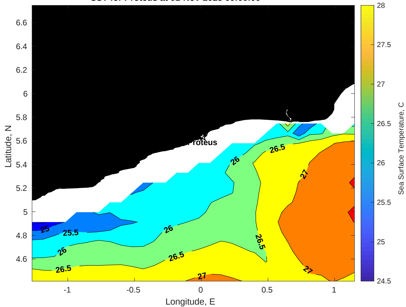
SST for Proteus at 01-Nov-2025 00:00:00
