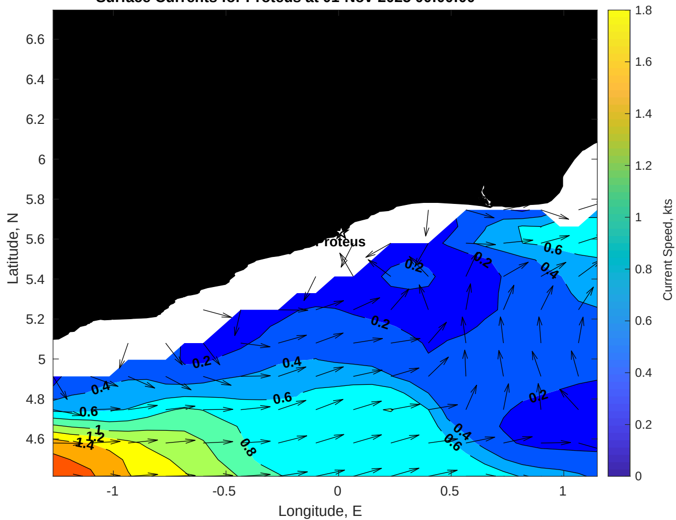
Surface Currents for Proteus at 01-Nov-2025 00:00:00
